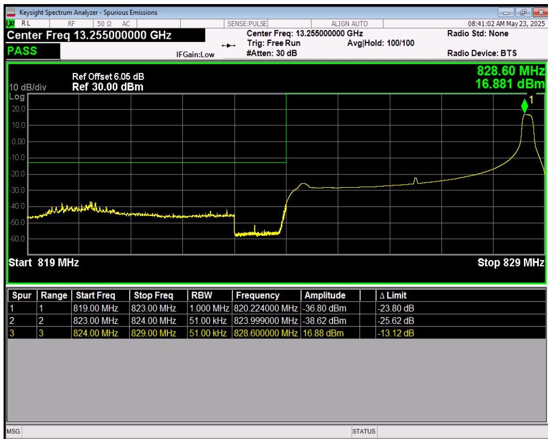
Band5 64QAM BW=5MHz Channel=20425 RB Size=1 Position=#0
