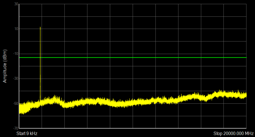
Band25 16QAM BW=5MHz Channel=26365 RB Size=25 Position=#0
