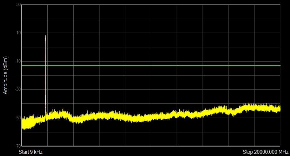
Band25 16QAM BW=15MHz Channel=26115 RB Size=75 Position=#0
