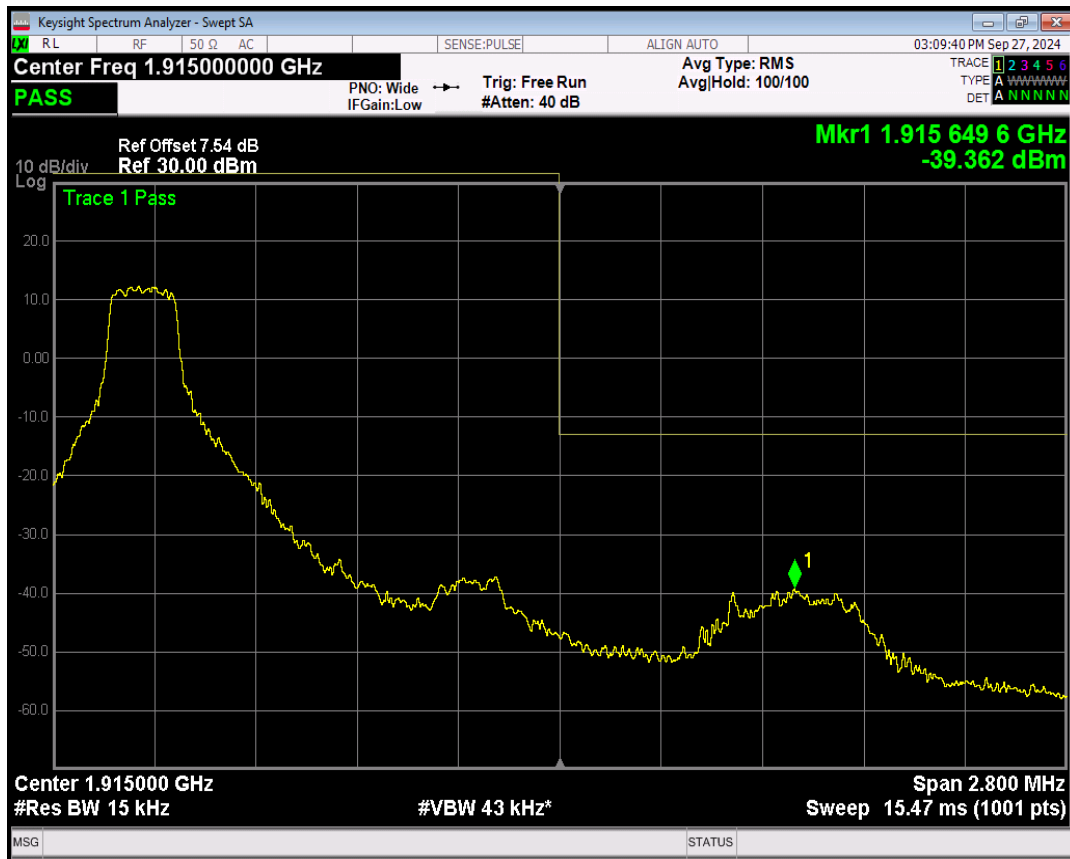
Band25 16QAM BW=1.4MHz Channel=26683 RB Size=1 Position=#Max
