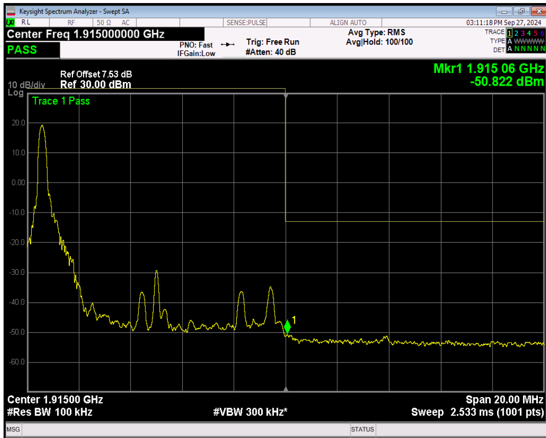
Band25 16QAM BW=10MHz Channel=26640 RB Size=1 Position=#Max
