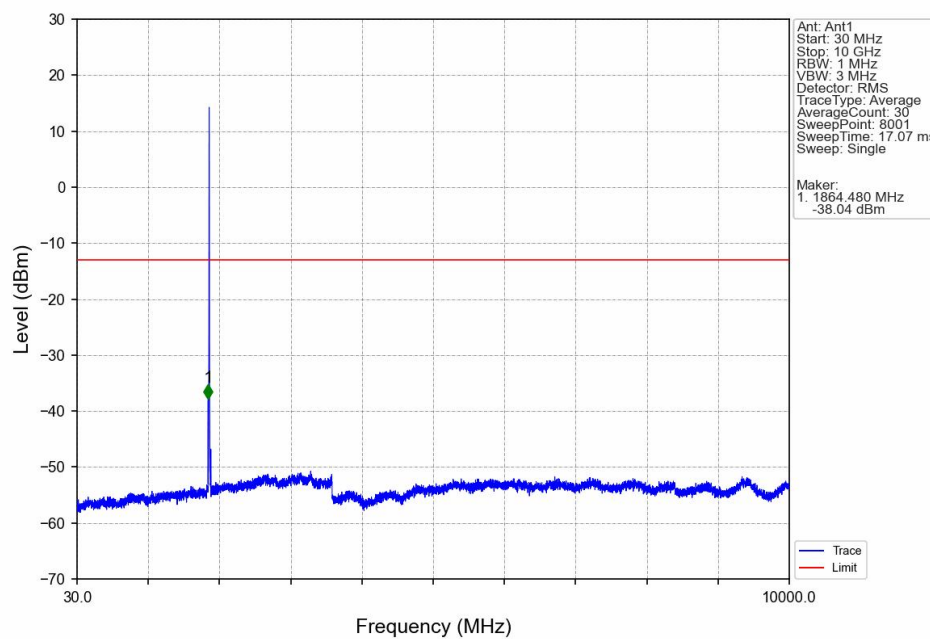
Band2_HSDPA_MCH_1880MHz_Subtest 1_NTNV
