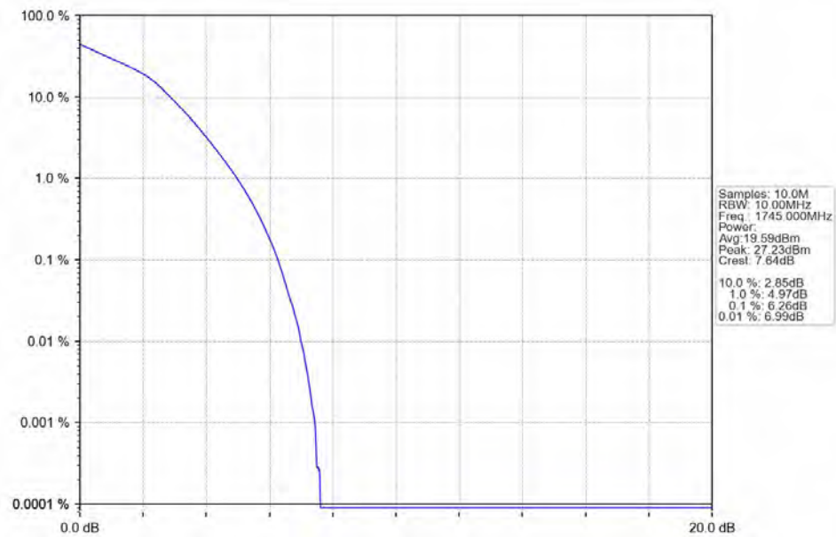
Band66_10MHz_16QAM_MCH_1745MHz_RB_50_0_NTNV
