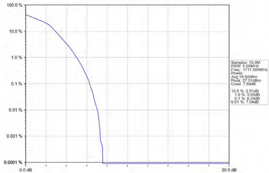
Band66_3MHz_16QAM_LCH_1711.5MHz_RB_15_0_NTNV
