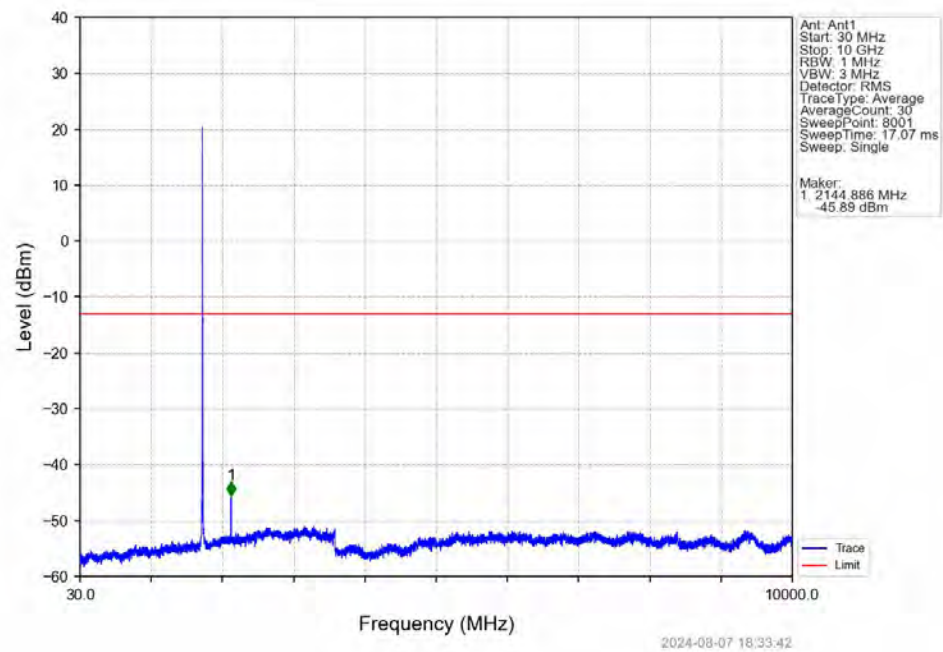
Band66_5MHz_16QAM_MCH_1745MHz_RB_1_0_NTNV
