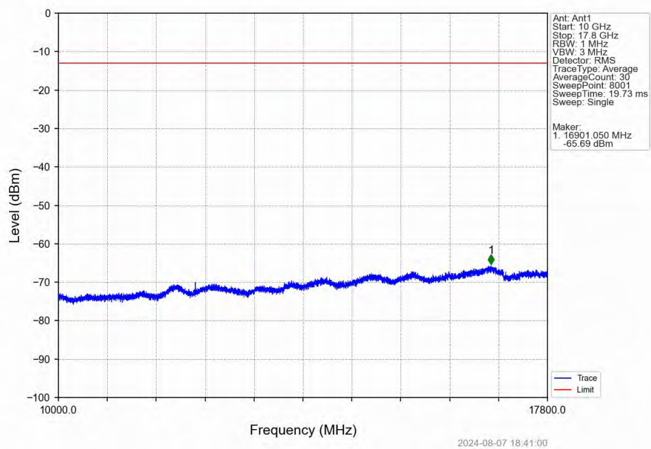
Band66_10MHz_QPSK_MCH_1745MHz_RB_1_0_NTNV
