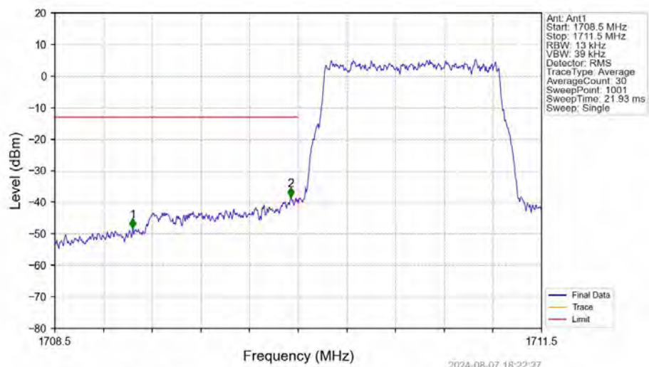
Band66_1.4MHz_QPSK_LCH_1710.7MHz_RB_6_0_NTNV
