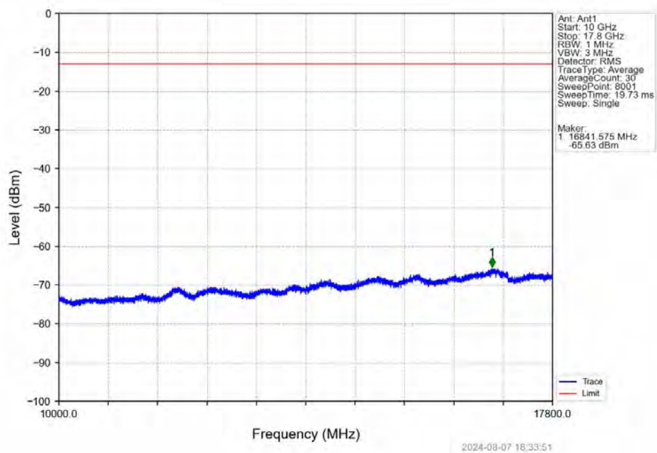
Band66_5MHz_16QAM_MCH_1745MHz_RB_1_0_NTNV
