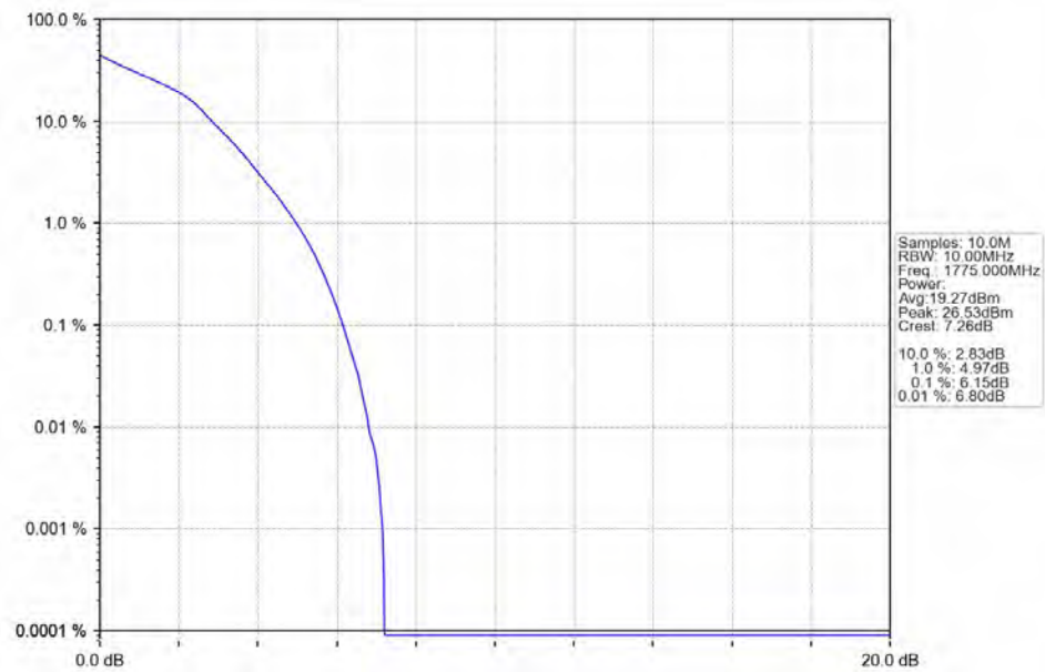
Band66_10MHz_16QAM_HCH_1775MHz_RB_50_0_NTNV
