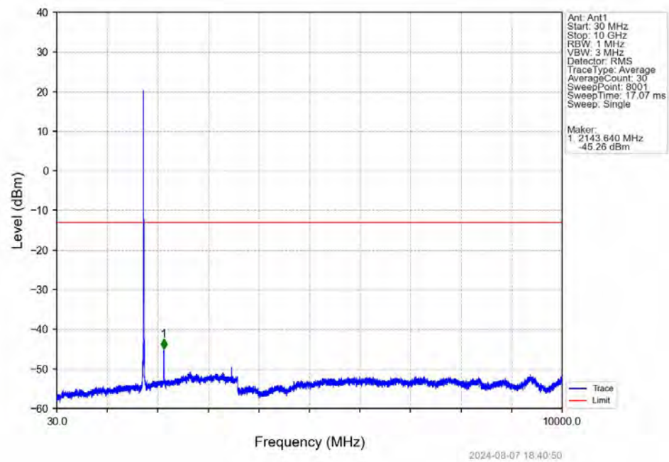
Band66_10MHz_QPSK_MCH_1745MHz_RB_1_0_NTNV
