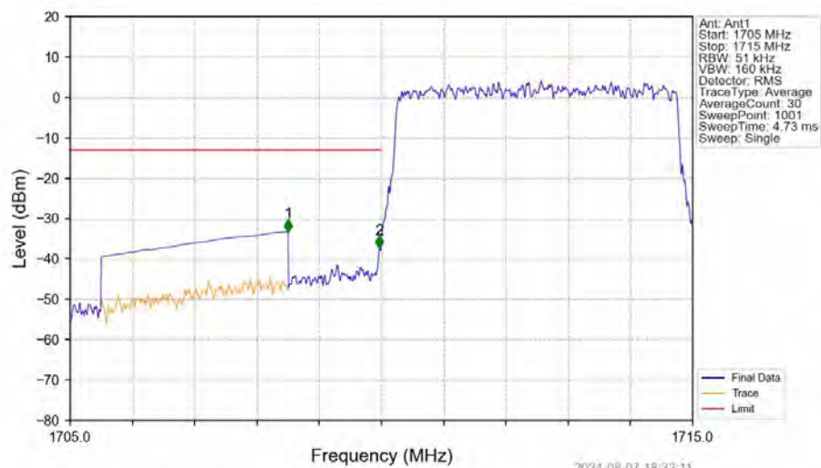
Band66_5MHz_16QAM_LCH_1712.5MHz_RB_25_0_NTNV
