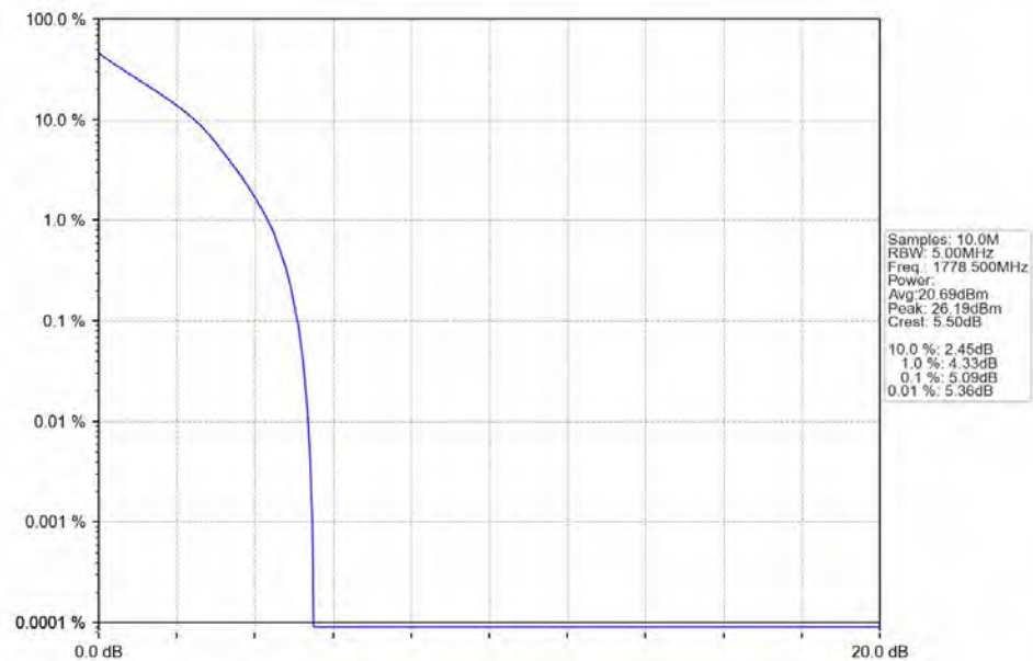
Band66_3MHz_QPSK_HCH_1778.5MHz_RB_15_0_NTNV
