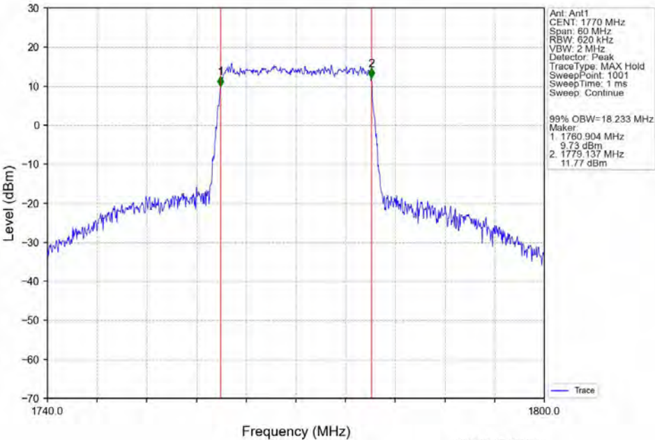
Band66_20MHz_16QAM_HCH_1770MHz_RB_100_0_NTNV
