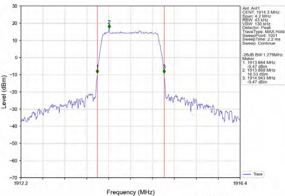
Band25_1.4MHz_16QAM_HCH_1914.3MHz_RB 6_0_NTNV
