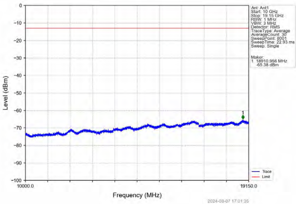
Band25_1.4MHz_QPSK_LCH_1850.7MHz_RB_6_0_NTNV
