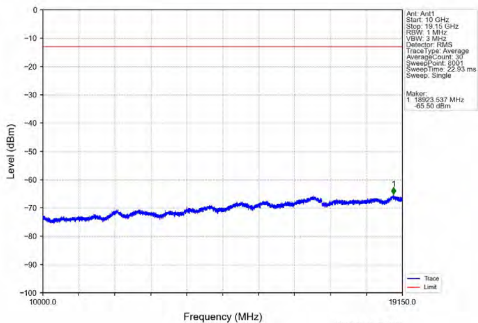
Band25_20MHz_16QAM_MCH_1882.5MHz_RB_1_0_NTNV
