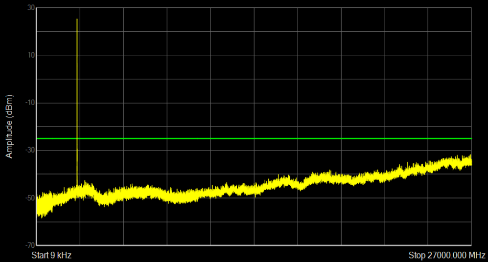
Band7 16QAM BW=5MHz Channel=21100 RB Size=1 Position=#0
