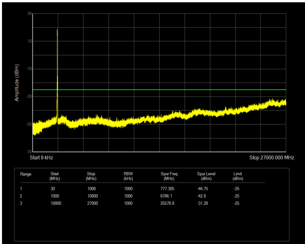
Band41(2545-2655) 16QAM BW=20MHz Channel=41140 RB Size=100 Position=#0
