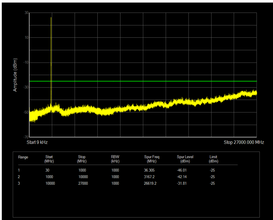
Band41(2545-2655) QPSK BW=5MHz Channel=40690 RB Size=25 Position=#0
