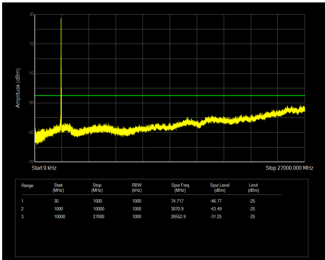
Band41(2545-2655) 16QAM BW=20MHz Channel=41140 RB Size=1 Position=#0
