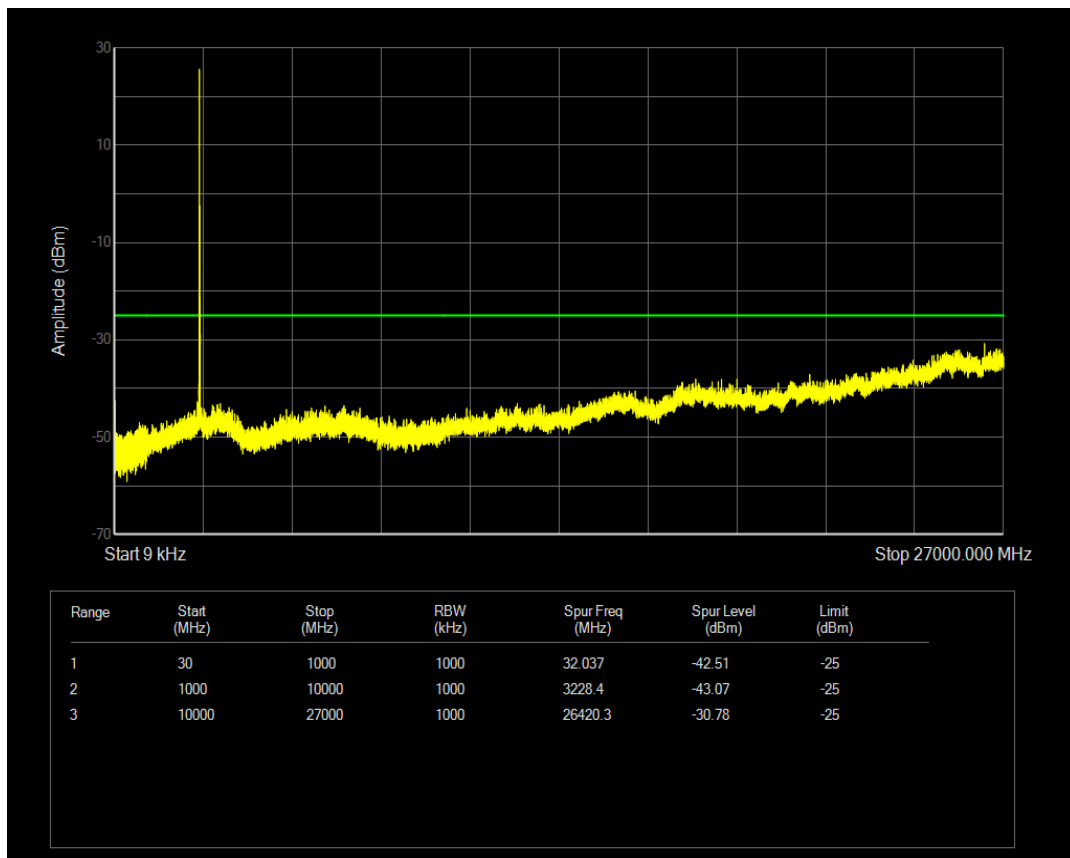
Band41(2545-2655) 16QAM BW=15MHz Channel=40690 RB Size=75 Position=#0
