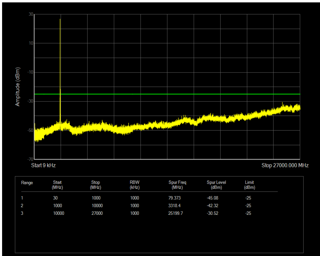
Band41(2545-2655) QPSK BW=15MHz Channel=41165 RB Size=75 Position=#0
