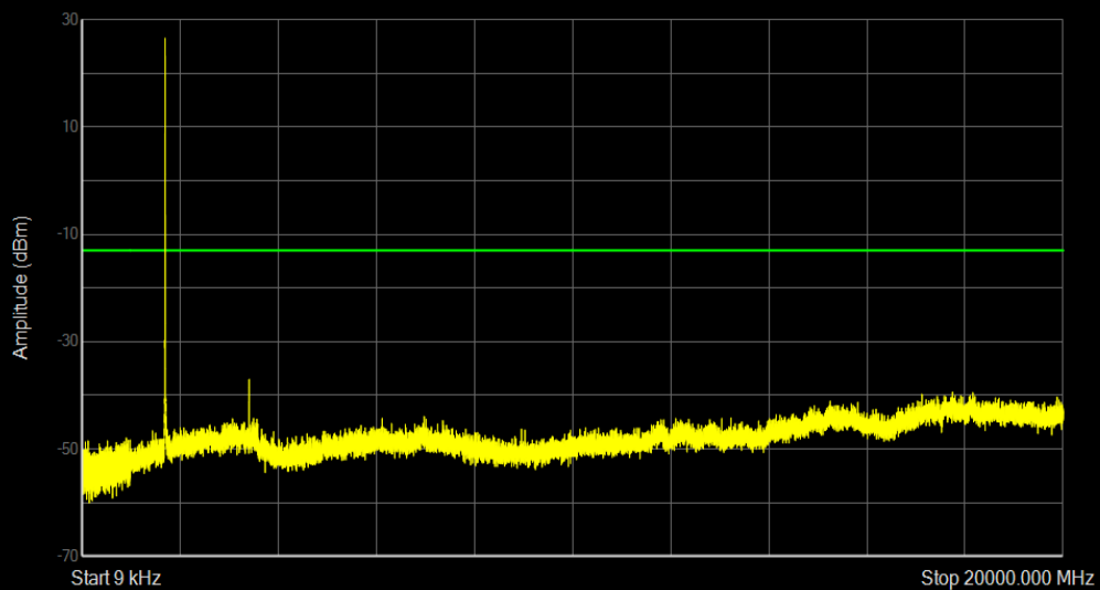
Band4 16QAM BW=3MHz Channel=19965 RB Size=1 Position=#0
