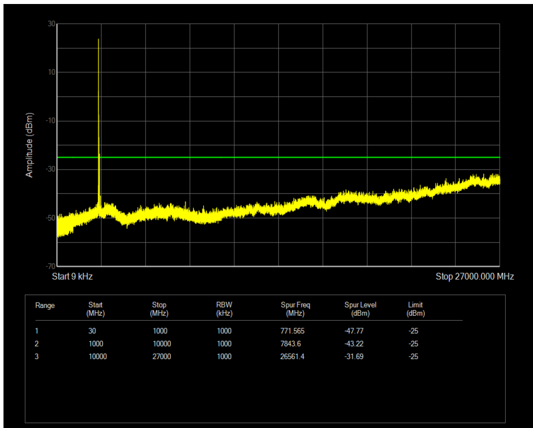
Band41(2545-2655) 16QAM BW=15MHz Channel=40215 RB Size=75 Position=#0
