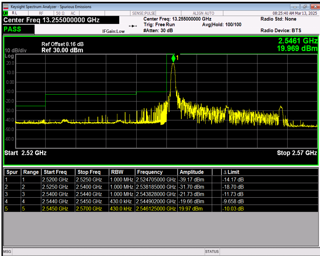
Band41(2545-2655) QPSK BW=20MHz Channel=40240 RB Size=1 Position=#Max
