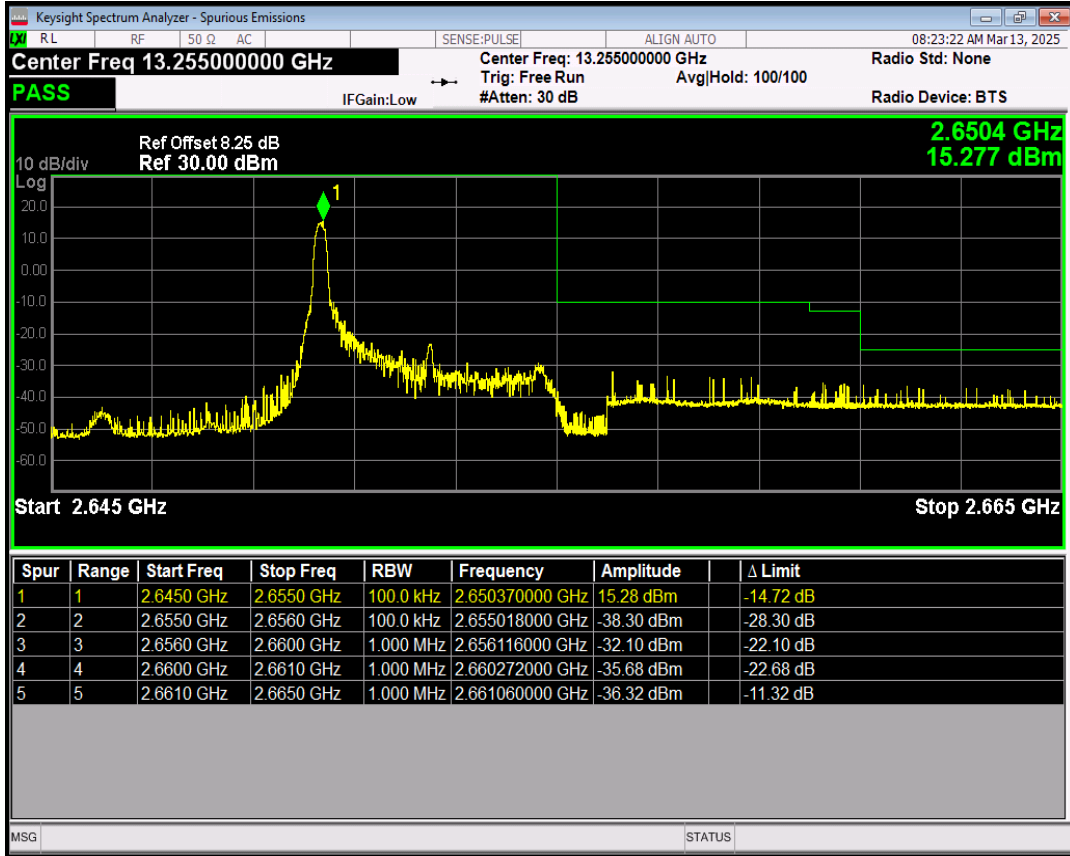
Band41(2545-2655) 16QAM BW=5MHz Channel=41215 RB Size=1 Position=#Max
