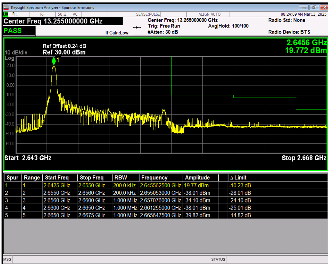
Band41(2545-2655) QPSK BW=10MHz Channel=41190 RB Size=1 Position=#Max
