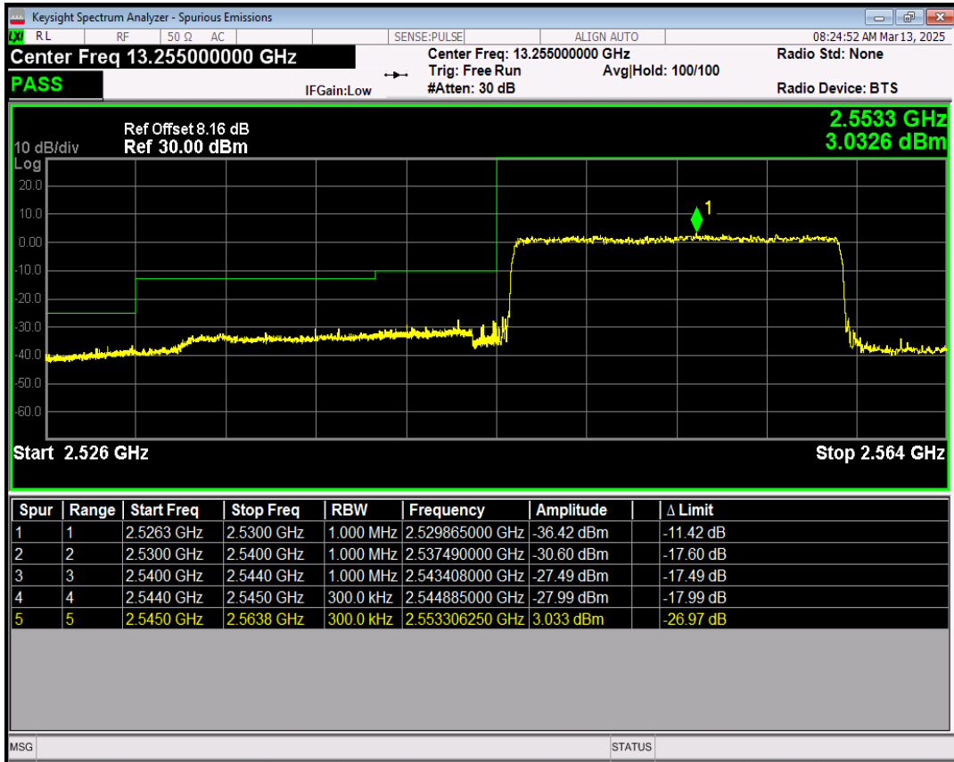
Band41(2545-2655) 16QAM BW=15MHz Channel=40215 RB Size=1 Position=#0
