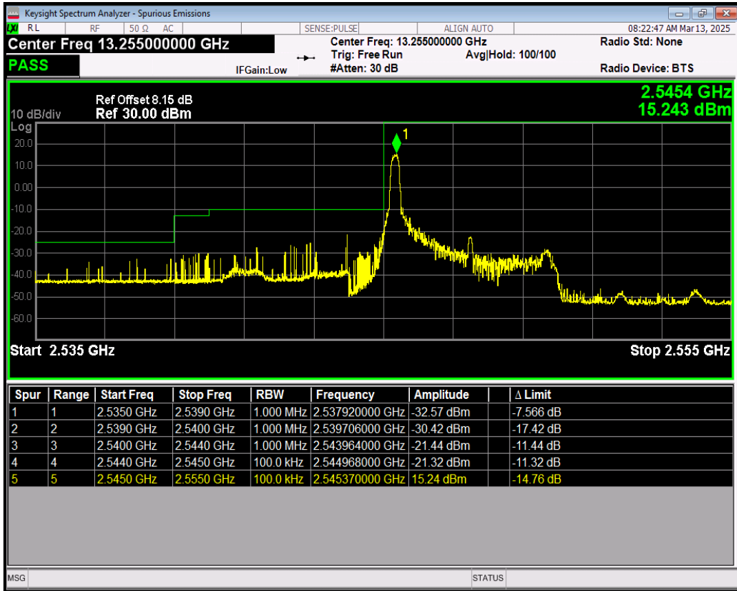
Band41(2545-2655) 16QAM BW=5MHz Channel=40165 RB Size=1 Position=#Max
