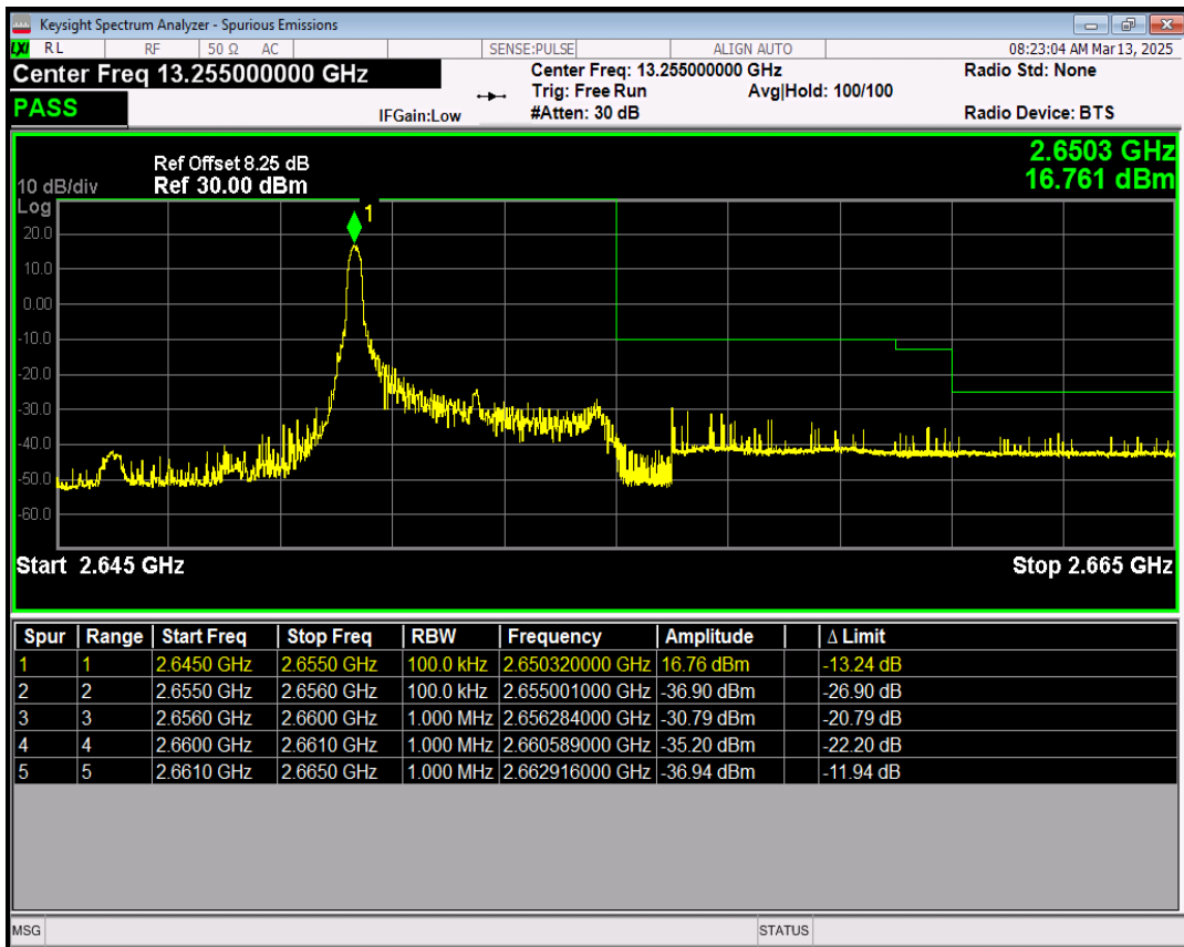
Band41(2545-2655) QPSK BW=5MHz Channel=41215 RB Size=1 Position=#Max
