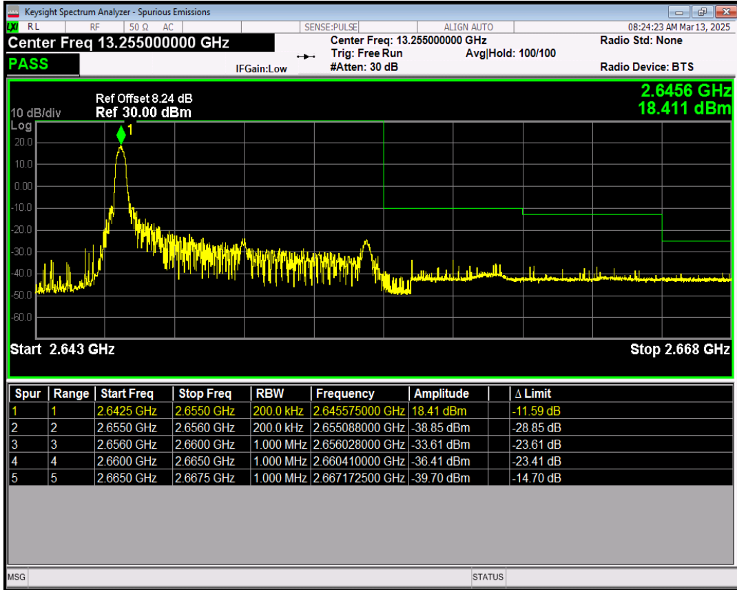
Band41(2545-2655) 16QAM BW=10MHz Channel=41190 RB Size=1 Position=#Max
