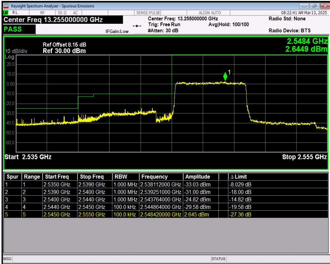
Band41(2545-2655) 16QAM BW=5MHz Channel=40165 RB Size=1 Position=#0
