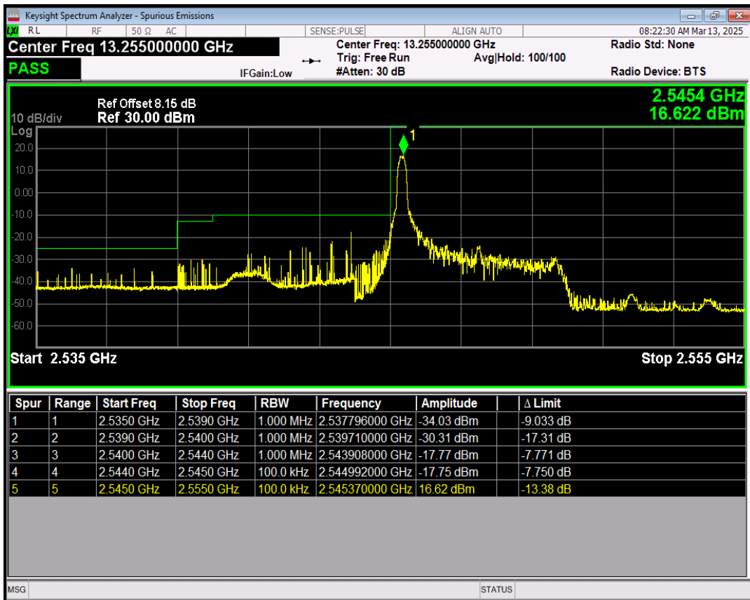
Band41(2545-2655) QPSK BW=5MHz Channel=40165 RB Size=1 Position=#Max
