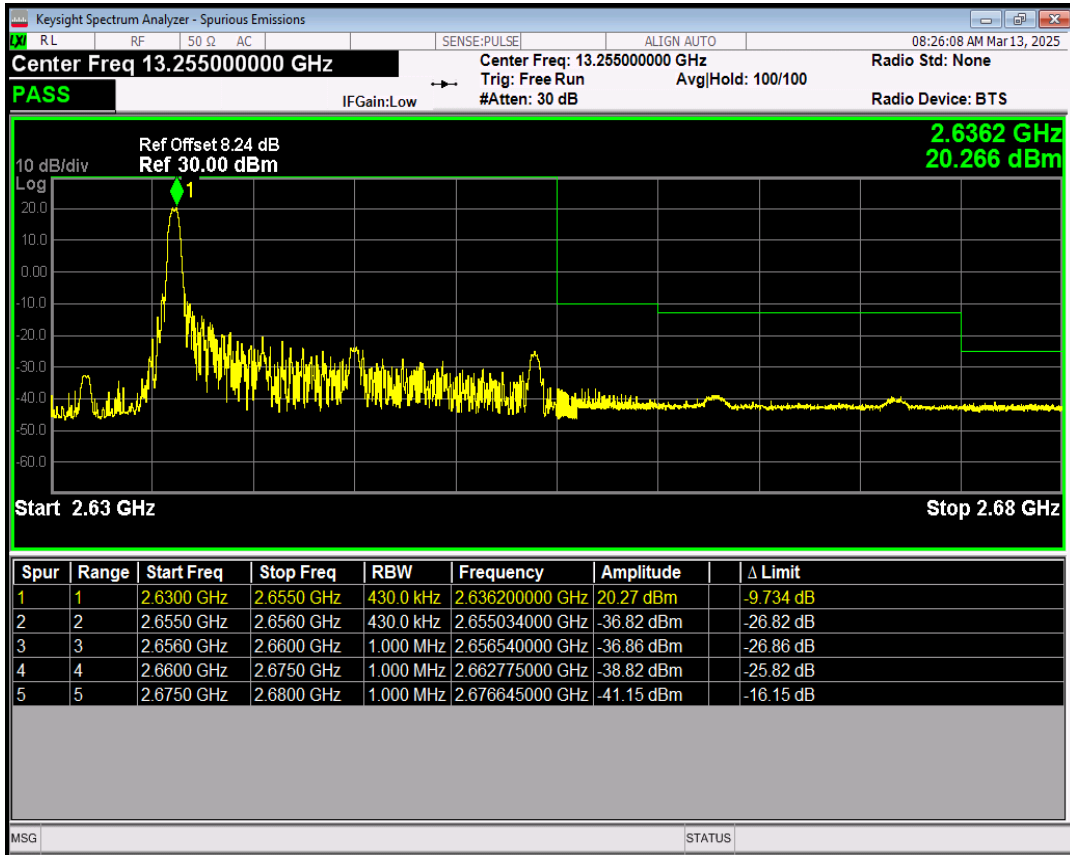
Band41(2545-2655) QPSK BW=20MHz Channel=41140 RB Size=1 Position=#Max
