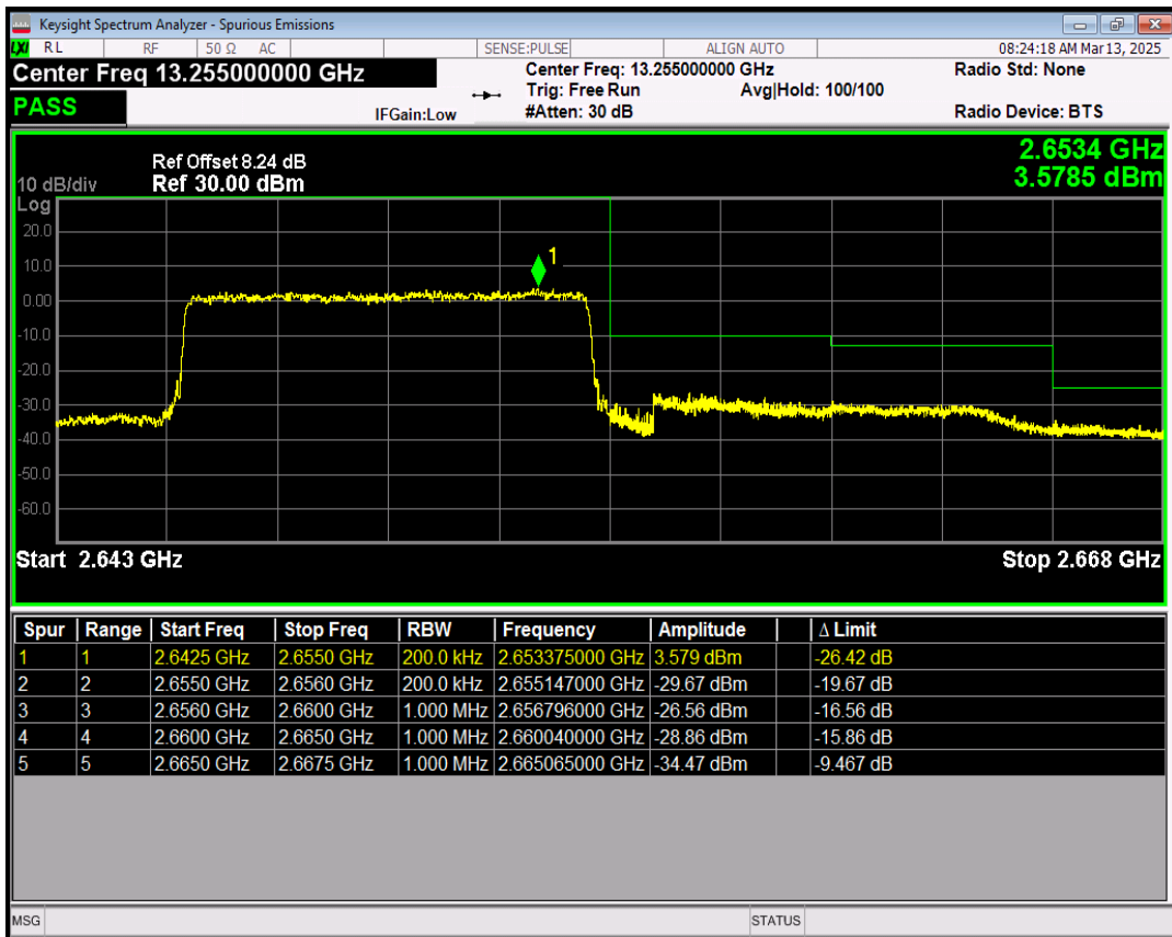
Band41(2545-2655) 16QAM BW=10MHz Channel=41190 RB Size=1 Position=#0
