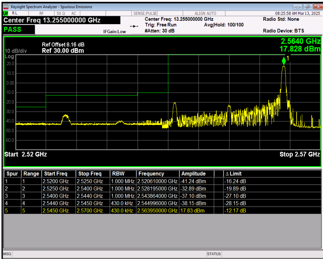
Band41(2545-2655) 16QAM BW=20MHz Channel=40240 RB Size=100 Position=#0
