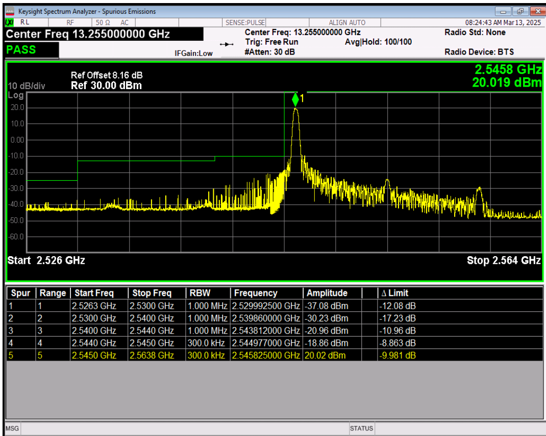
Band41(2545-2655) QPSK BW=15MHz Channel=40215 RB Size=1 Position=#Max
