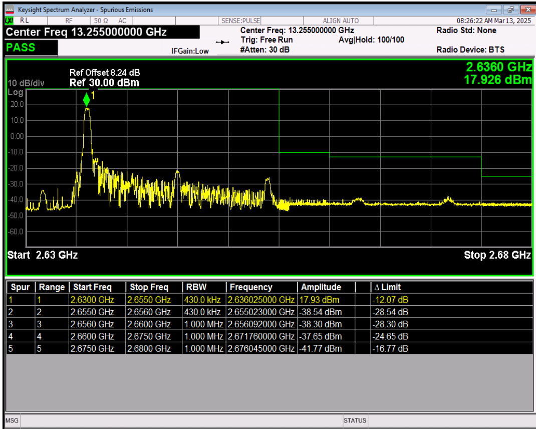
Band41(2545-2655) 16QAM BW=20MHz Channel=41140 RB Size=1 Position=#Max
