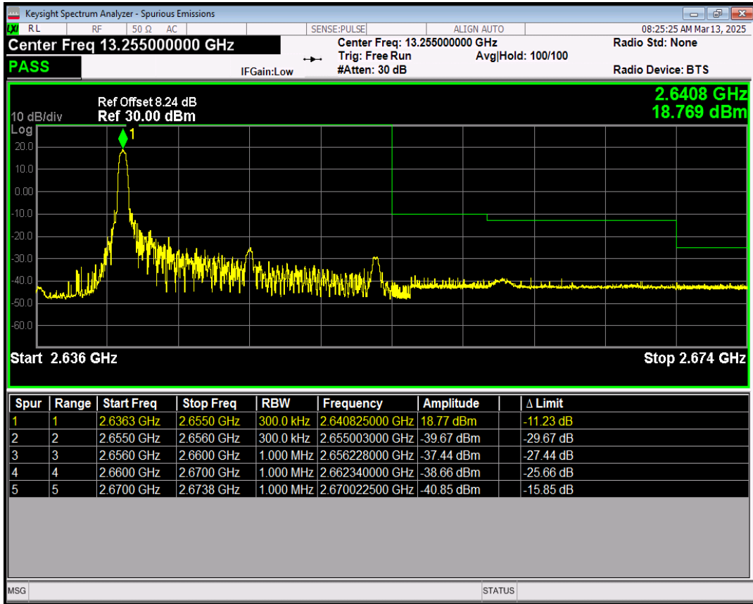
Band41(2545-2655) 16QAM BW=15MHz Channel=41165 RB Size=1 Position=#Max
