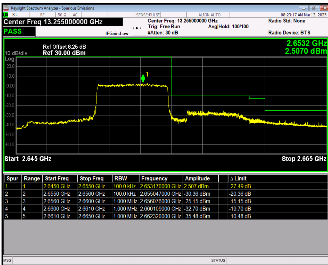
Band41(2545-2655) 16QAM BW=5MHz Channel=41215 RB Size=1 Position=#0
