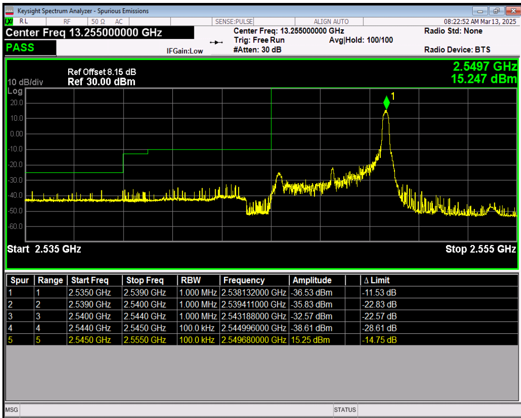
Band41(2545-2655) 16QAM BW=5MHz Channel=40165 RB Size=25 Position=#0
