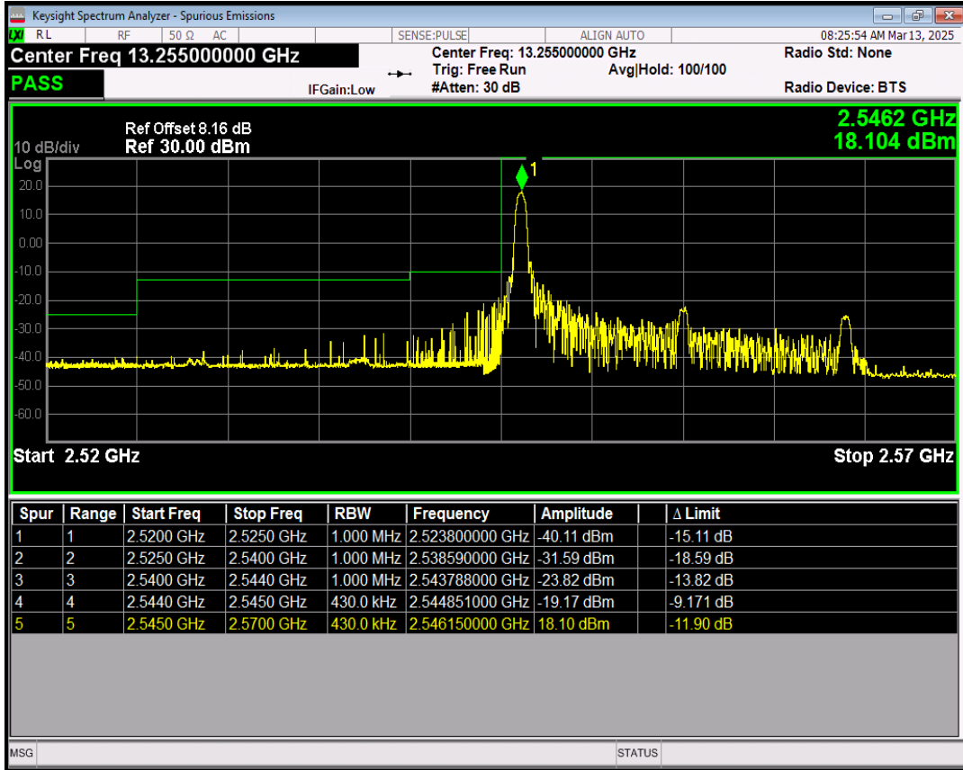
Band41(2545-2655) 16QAM BW=20MHz Channel=40240 RB Size=1 Position=#Max
