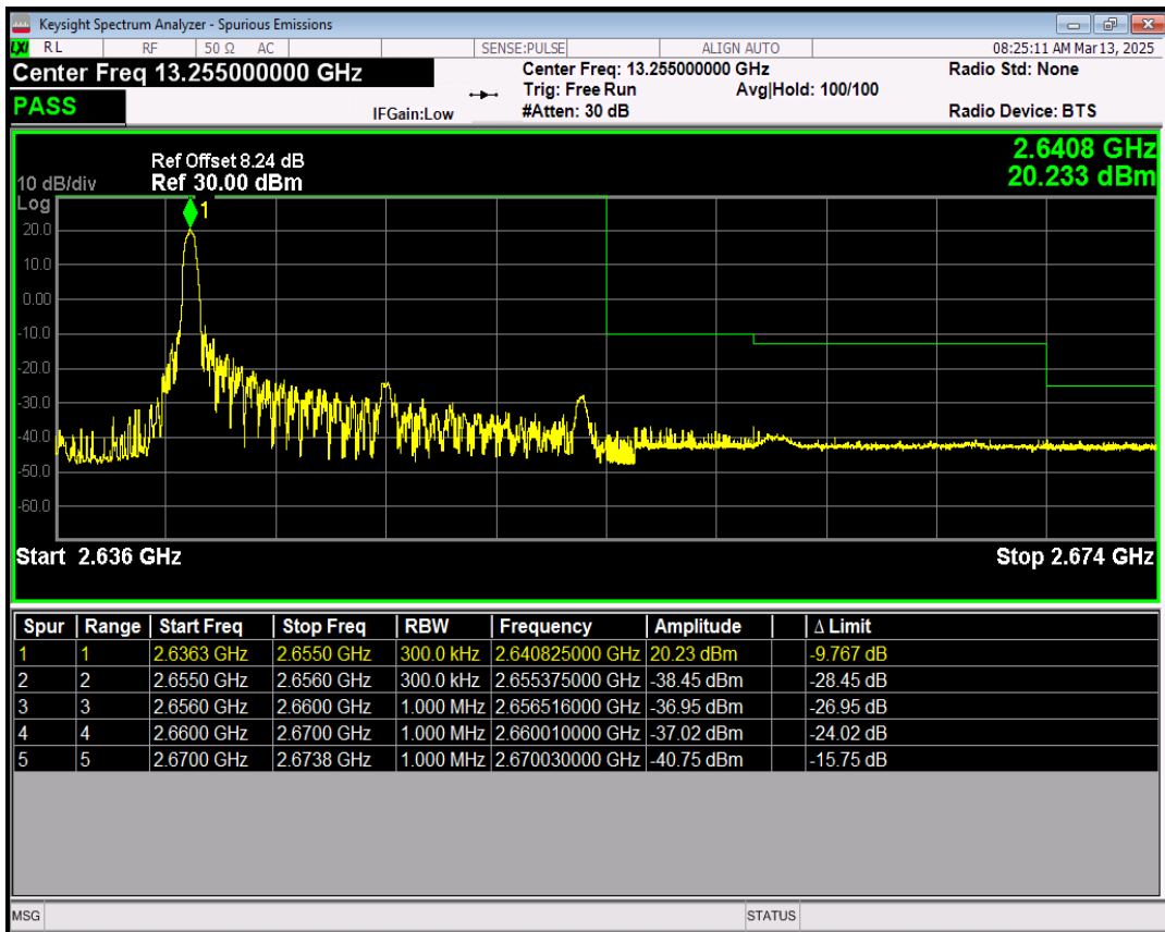
Band41(2545-2655) QPSK BW=15MHz Channel=41165 RB Size=1 Position=#Max
