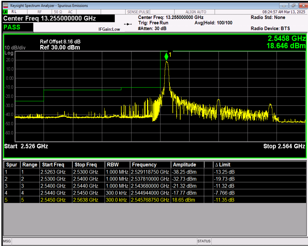
Band41(2545-2655) 16QAM BW=15MHz Channel=40215 RB Size=1 Position=#Max
