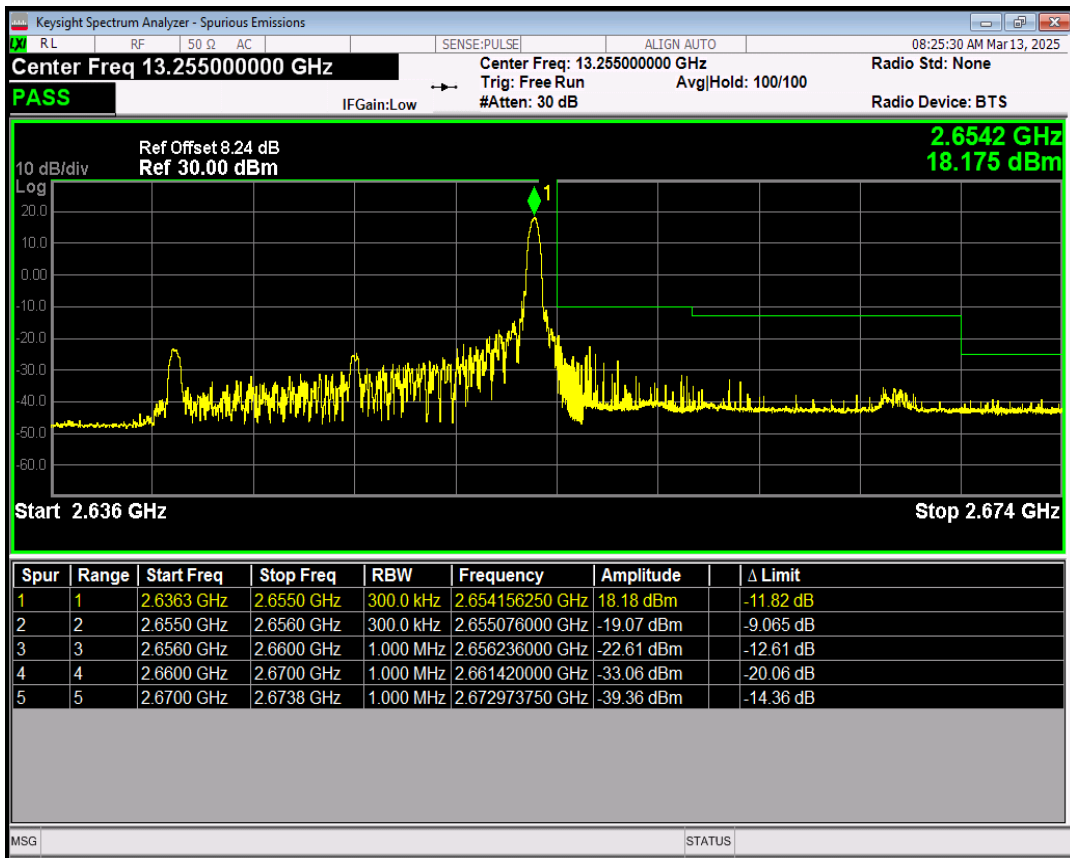
Band41(2545-2655) 16QAM BW=15MHz Channel=41165 RB Size=75 Position=#0
