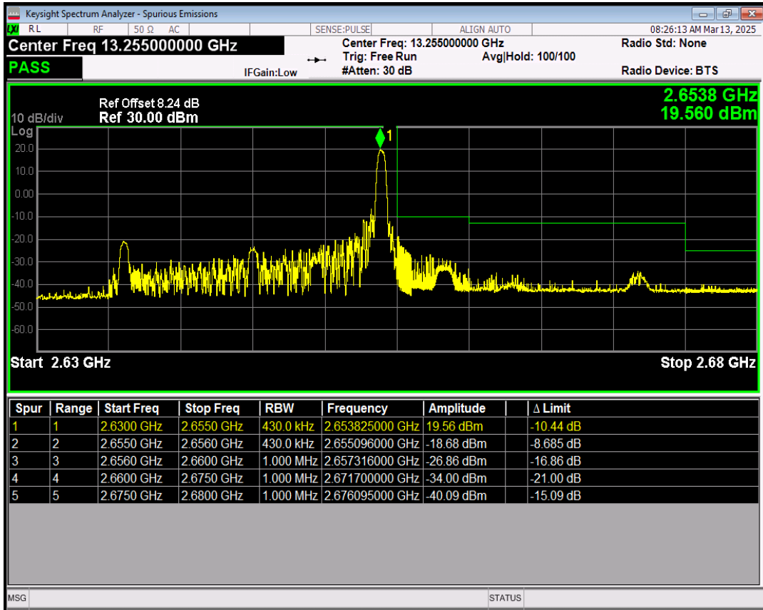
Band41(2545-2655) QPSK BW=20MHz Channel=41140 RB Size=100 Position=#0
