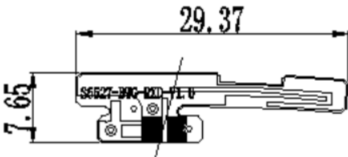
Diversity Antenna
