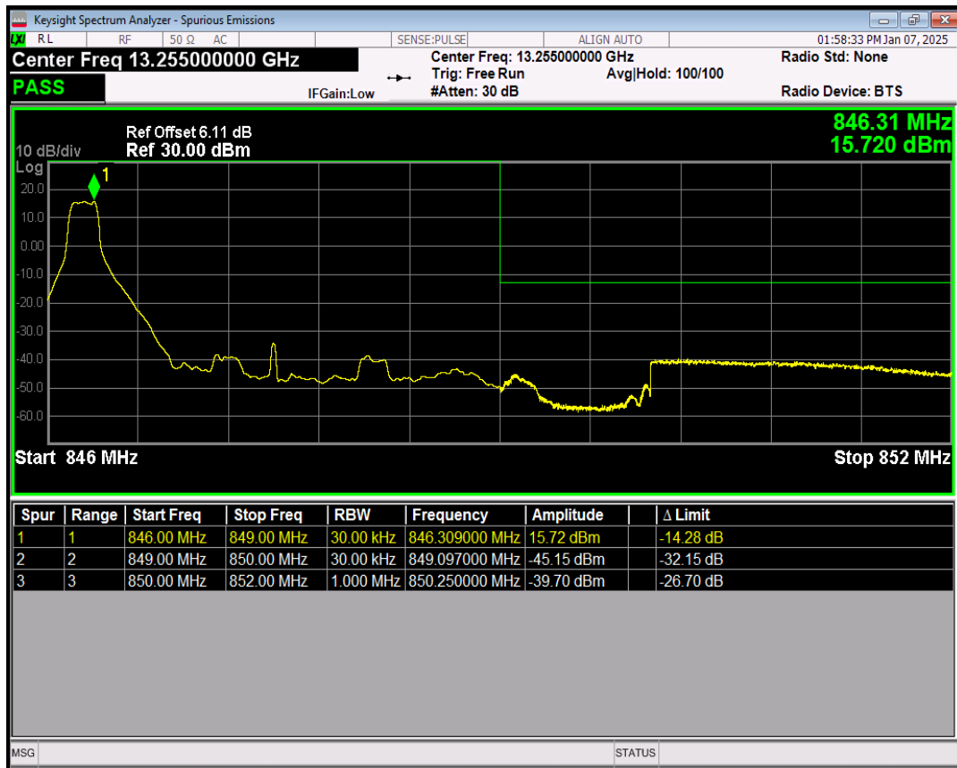
Band26(824-849) QPSK BW=3MHz Channel=27025 RB Size=1 Position=#Max
