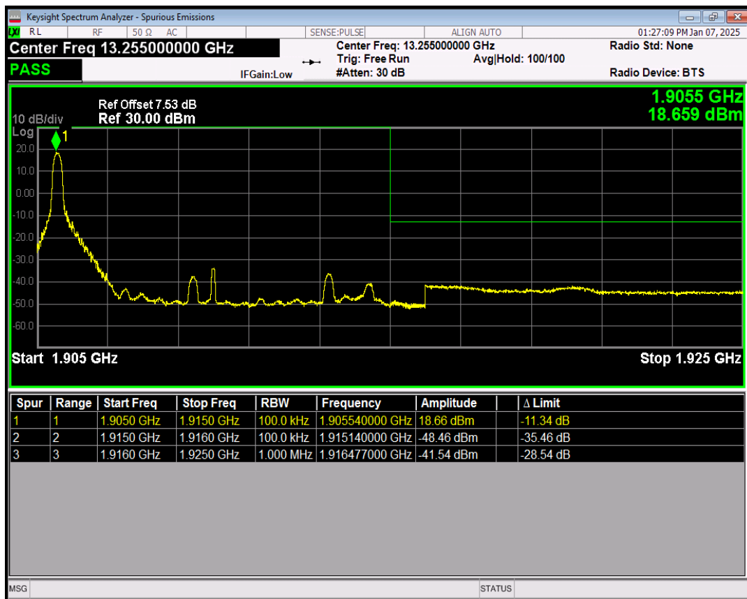
Band25 16QAM BW=10MHz Channel=26640 RB Size=1 Position=#Max
