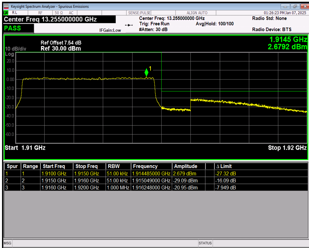
Band25 16QAM BW=5MHz Channel=26665 RB Size=1 Position=#Max
