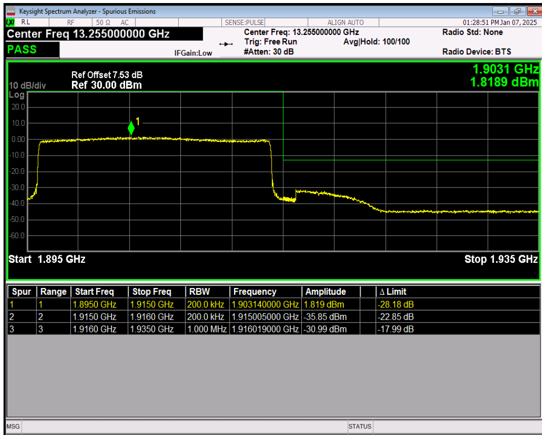
Band25 16QAM BW=20MHz Channel=26590 RB Size=1 Position=#Max
