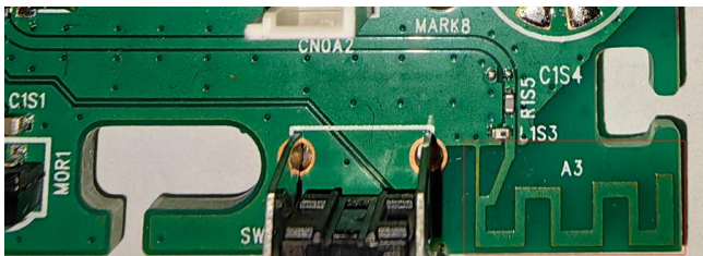
Bluetooth antenna
