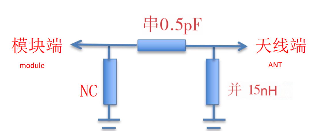
Antenna Matching Circuit Diagram
