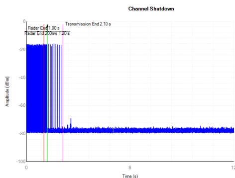
5530MHz Shutdown
