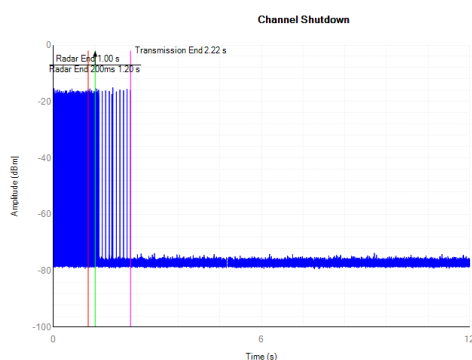
5290MHz Shutdown
