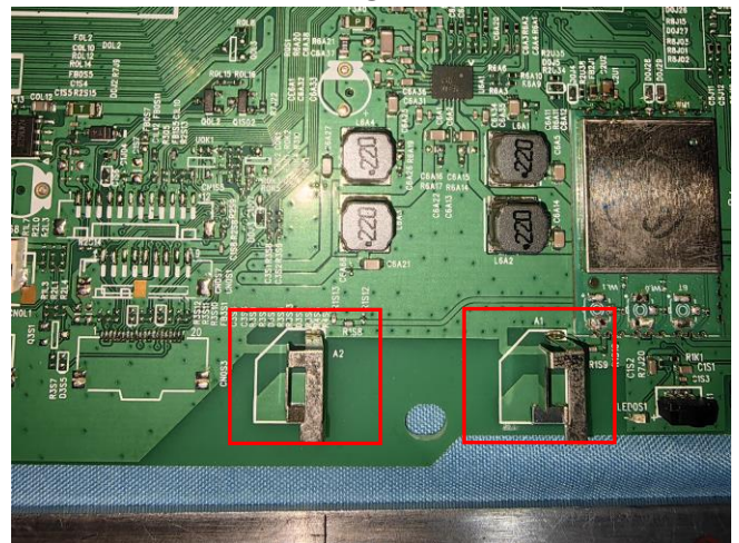
Wi-fi antenna(Front)
