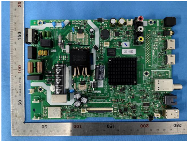
Test board 1
