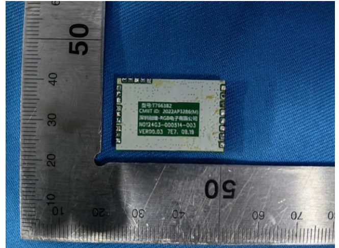
Side view 2
