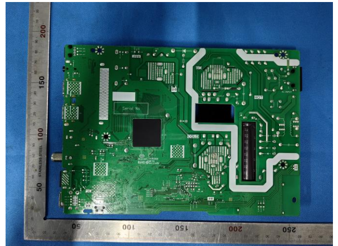
Test board 2
