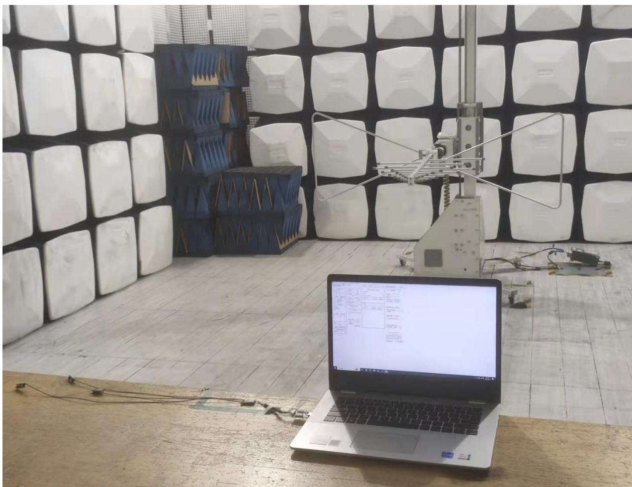
Photograph 1: Set-up for Radiated Spurious Emission, Below 1GHz
