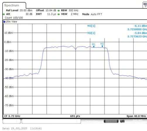
11AC20MIMO-Ant1-5720_UNII-3-PASS
