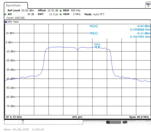
11AC20MIMO-Ant2-5720_UNII-3-PASS
