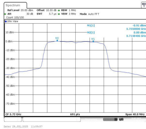
11A-CDD-Ant2-5720_UNII-2C-PASS
