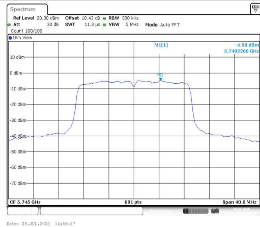
11AC20MIMO-Ant2-5745-PASS
