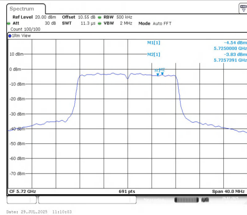
11A-CDD-Ant2-5720_UNII-3-PASS
