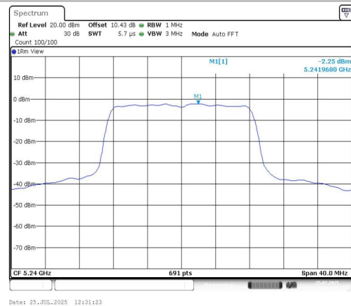
11A-CDD-Ant2-5240-PASS
