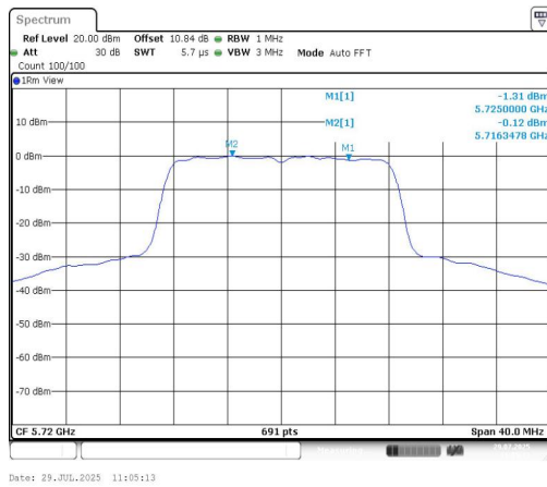
11A-CDD-Ant1-5720_UNII-2C-PASS
