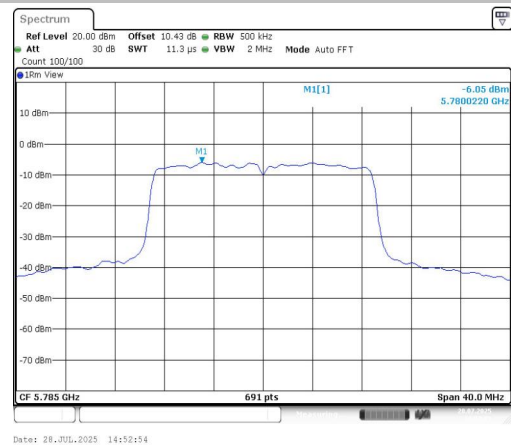
11AC20MIMO-Ant2-5785-PASS
