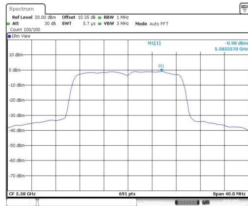
11AC20MIMO-Ant2-5580-PASS
