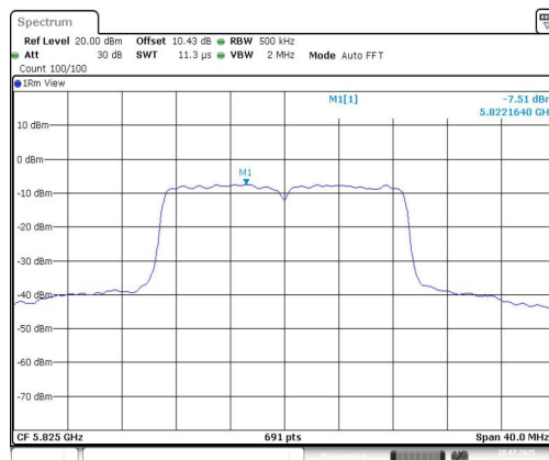
11AC20MIMO-Ant2-5825-PASS
