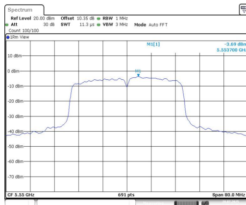
11AC40MIMO-Ant2-5550-PASS
