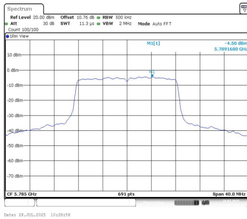
11A-CDD-Ant1-5785-PASS
