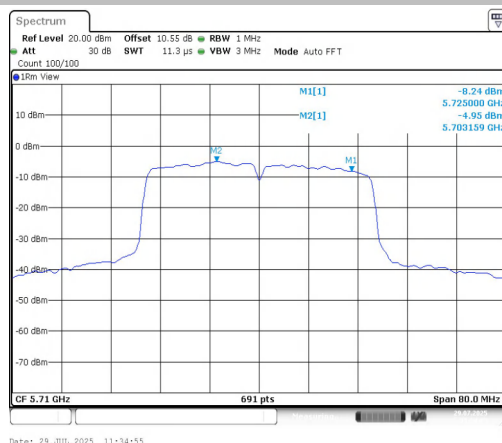
11AC40MIMO-Ant2-5710_UNII-2C-PASS
