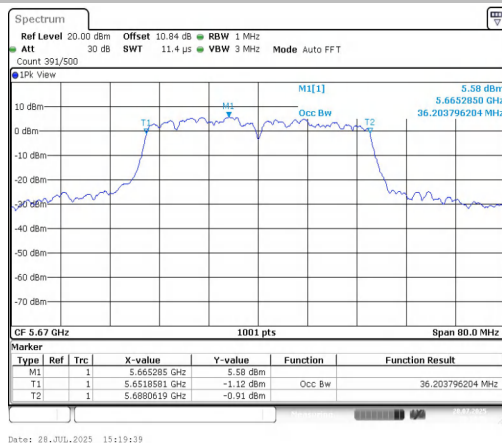
11AC40MIMO-Ant1-5670
