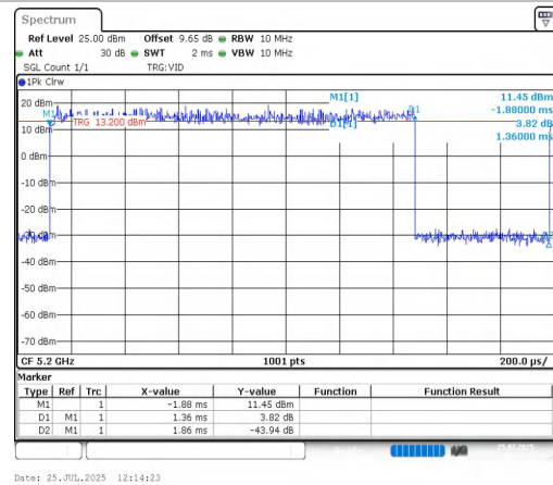
NTVN-11A-CDD-Ant2-5200
