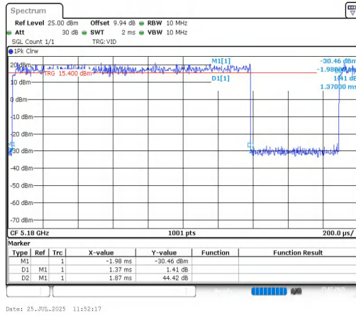
NTVN-11A-CDD-Ant1-5180
