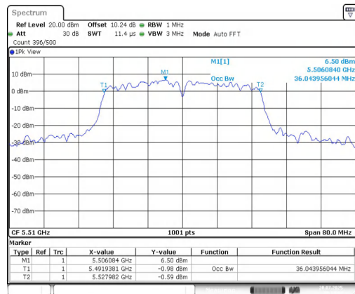
11AC40MIMO-Ant2-5510
