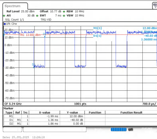
NTVN-11A-CDD-Ant1-5240
