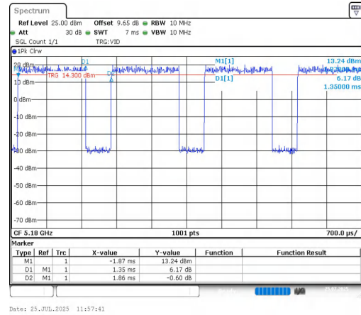
NTVN-11A-CDD-Ant2-5180
