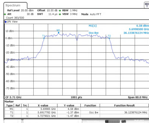
11AC40MIMO-Ant2-5710
