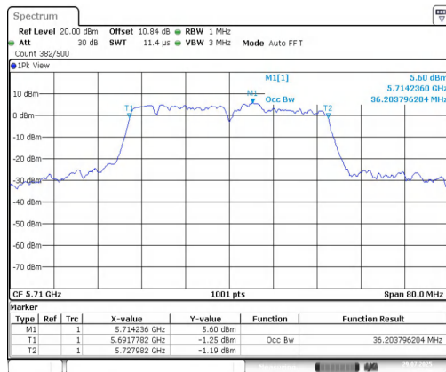
11AC40MIMO-Ant1-5710
