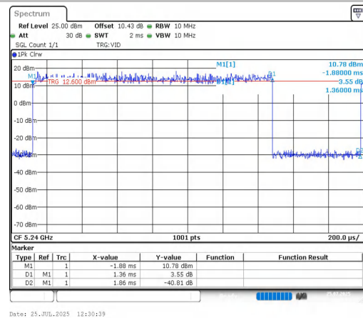
NTVN-11A-CDD-Ant2-5240
