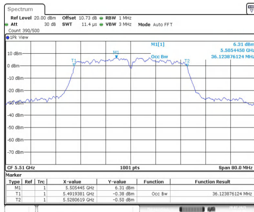
11AC40MIMO-Ant1-5510
