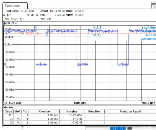
NTNV-11A-CDD-Ant1-5720
