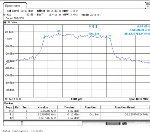
11AC40MIMO-Ant2-5670
