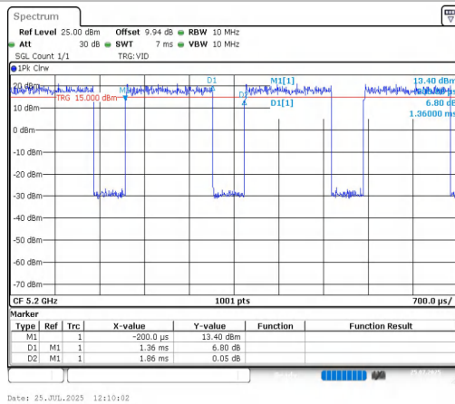
NTVN-11A-CDD-Ant1-5200
