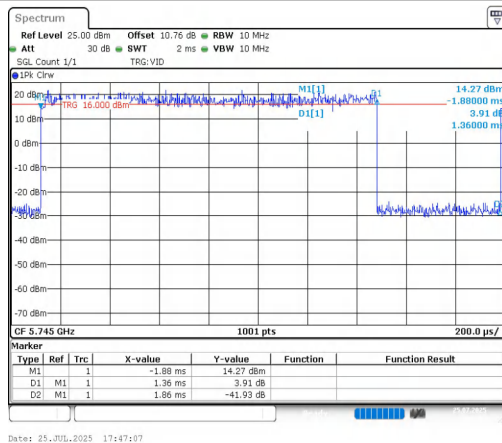
NTNV-11A-CDD-Ant1-5745
