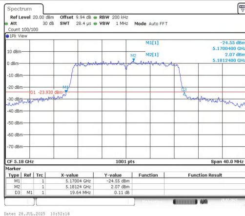
11AC20MIMO-Ant1-5180
