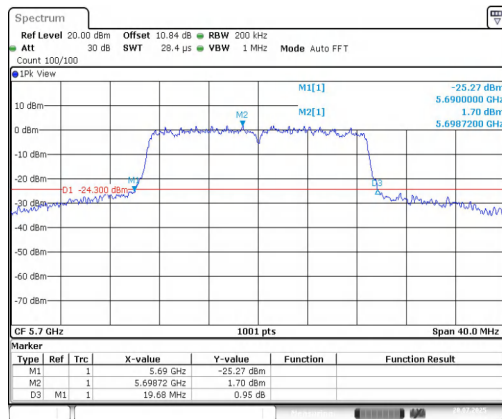
11AC20MIMO-Ant1-5700
