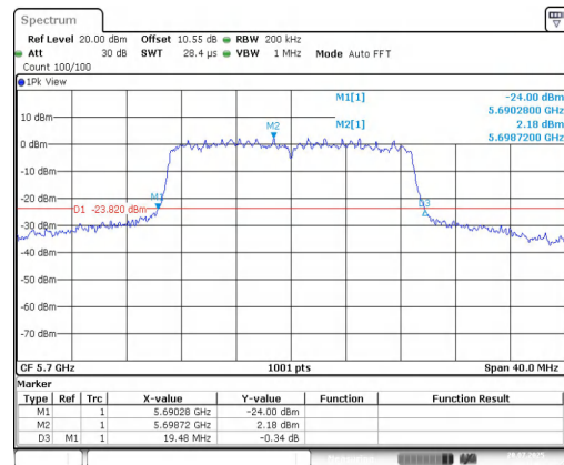
11AC20MIMO-Ant2-5700
