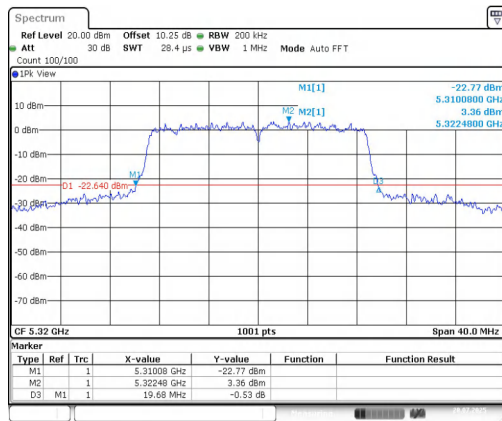
11AC20MIMO-Ant1-5320
