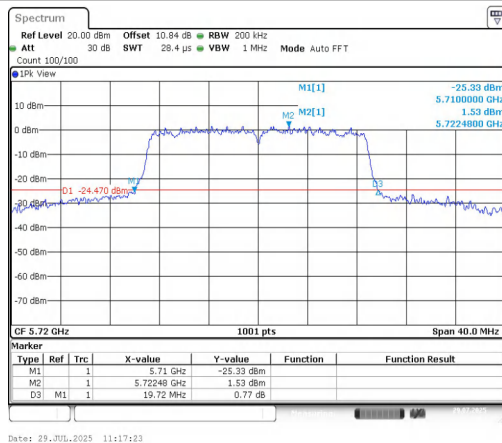
11AC20MIMO-Ant1-5720
