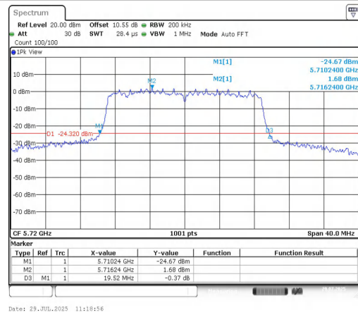
11AC20MIMO-Ant2-5720
