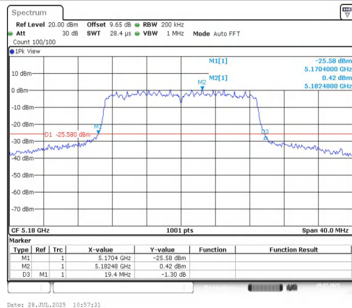
11AC20MIMO-Ant2-5180
