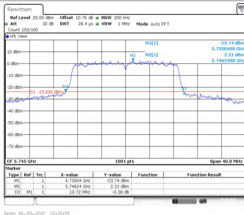
11AC20MIMO-Ant1-5745
