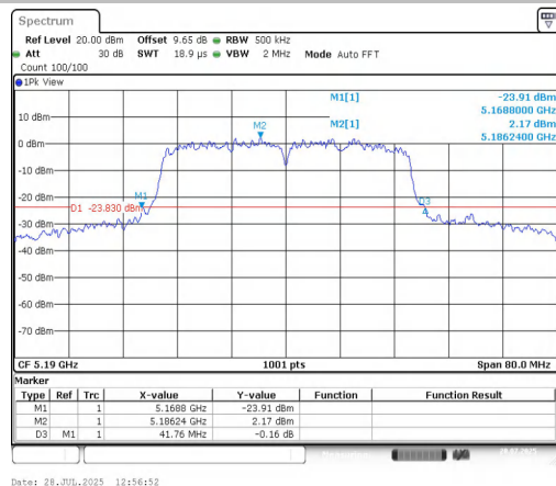
11AC40MIMO-Ant2-5190
