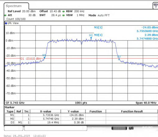
11AC20MIMO-Ant2-5745
