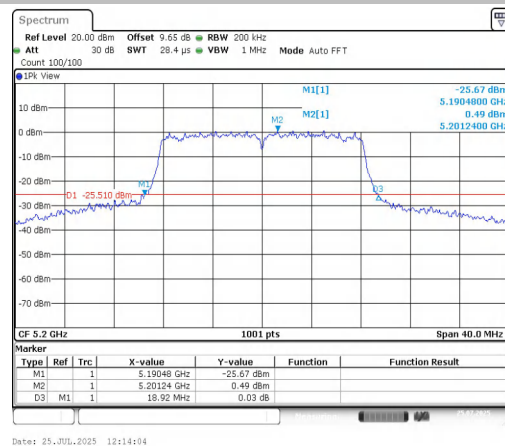
11A-CDD-Ant2-5200
