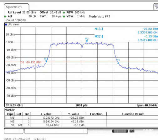
11A-CDD-Ant2-5240
