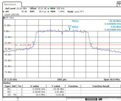
11AC20MIMO-Ant2-5320
