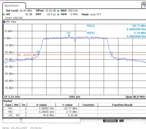
11AC40MIMO-Ant1-5310
