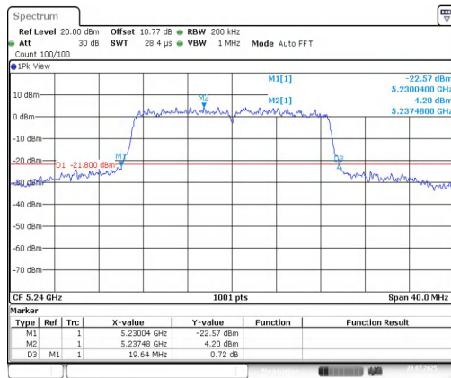
11AC20MIMO-Ant1-5240
