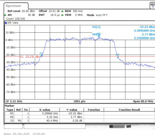
11AC40MIMO-Ant2-5310
