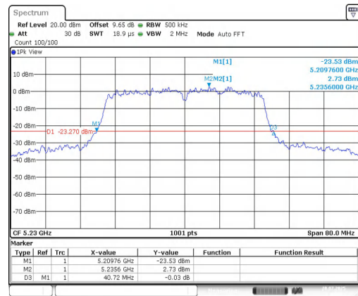
11AC40MIMO-Ant2-5230
