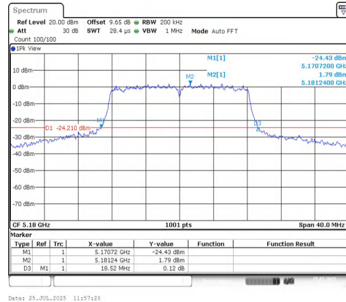
11A-CDD-Ant2-5180
