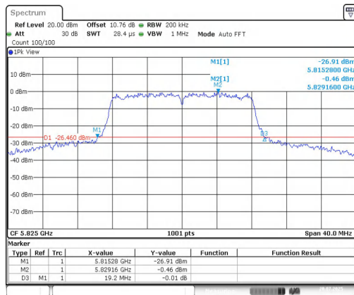
11A-CDD-Ant1-5825
