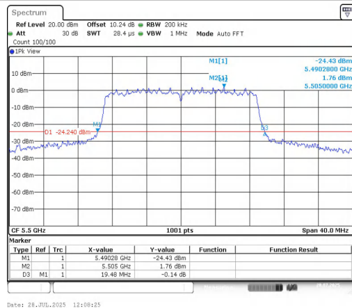
11AC20MIMO-Ant2-5500
