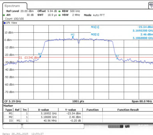
11AC40MIMO-Ant1-5190
