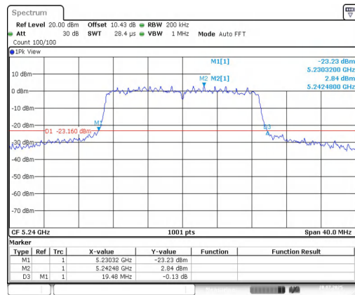
11AC20MIMO-Ant2-5240
