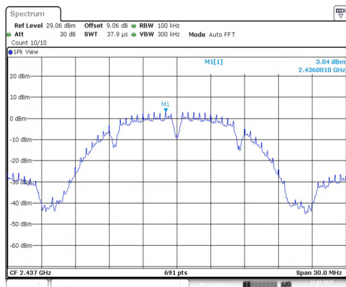
11B-CDD-Ant1-2437-0~Reference-PASS
