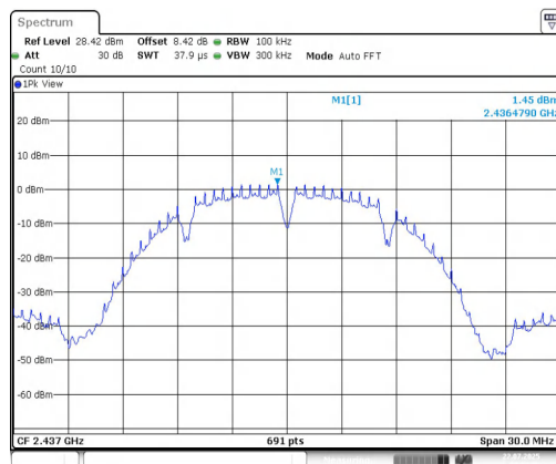
11B-CDD-Ant2-2437-0~Reference-PASS
