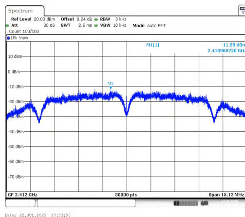
11B-CDD-Ant2-2412-PASS
