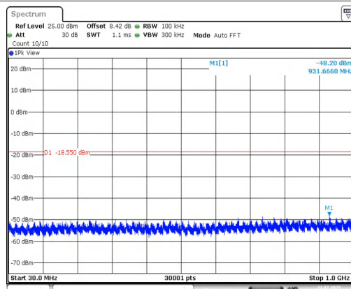
11B-CDD-Ant2-2437-0~Reference-PASS
