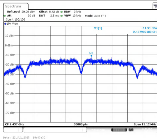
11B-CDD-Ant2-2437-PASS
