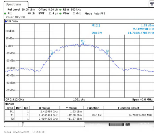
11B-CDD-Ant2-2412
