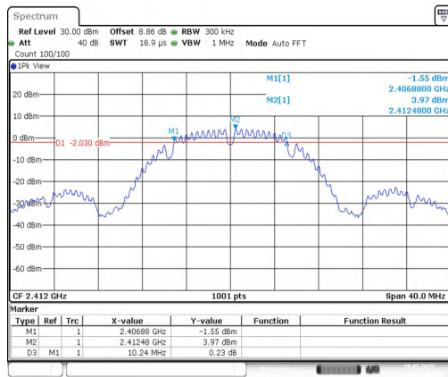
11B-CDD-Ant1-2412-PASS
