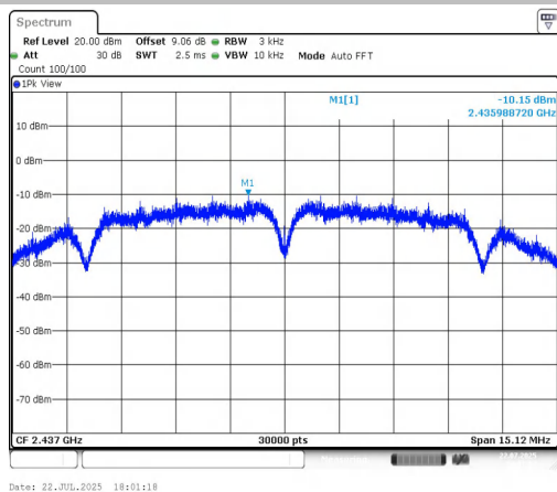
11B-CDD-Ant1-2437-PASS
