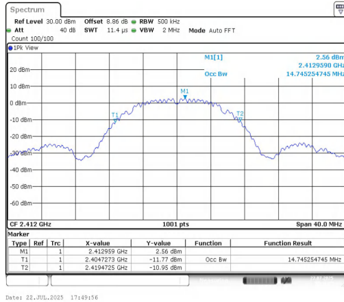
11B-CDD-Ant1-2412
