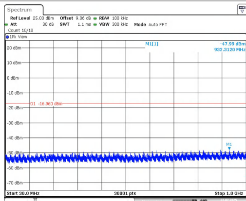
11B-CDD-Ant1-2437-0~Reference-PASS
