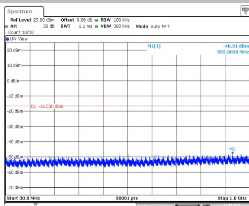
11B-CDD-Ant1-2462-0~Reference-PASS
