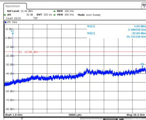
DH5-Ant1-2480-0~Reference-PASS
