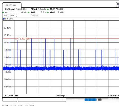
2D1-Ant1-Hop-PASS
