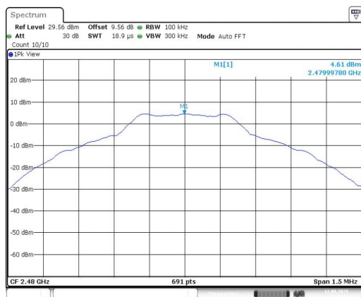
DH5-Ant1-2480-0~Reference-PASS
