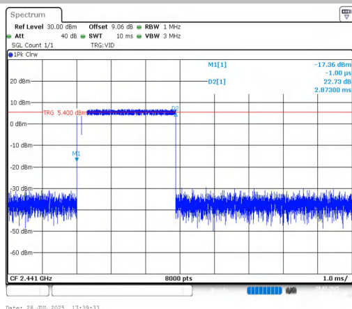
2D1-Ant1-Hop-PASS
