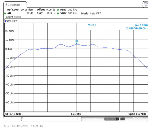
2DH5-Ant1-2480-0~Reference-PASS
