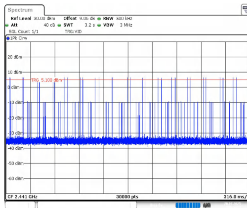
2D1-Ant1-Hop-PASS
