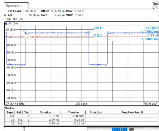
NTNV-3DH5-Ant1-2441
