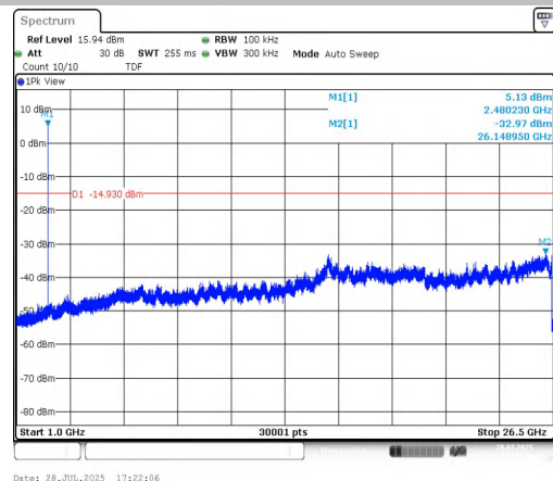
2DH5-Ant1-2480-1000~26500-PASS
