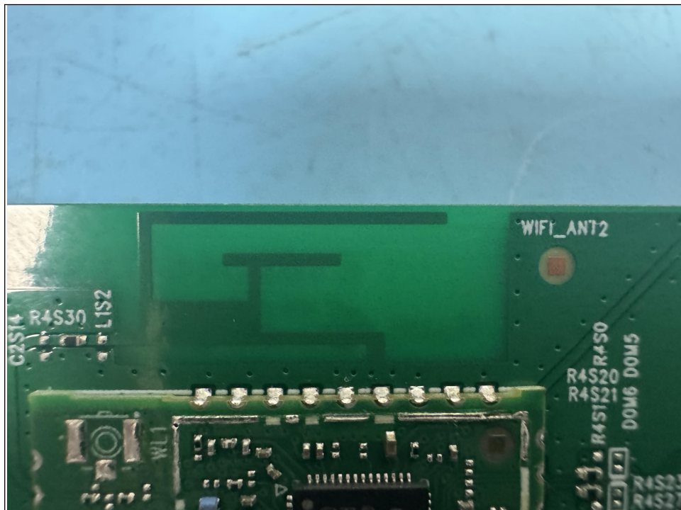
WiFi Antenna 2
