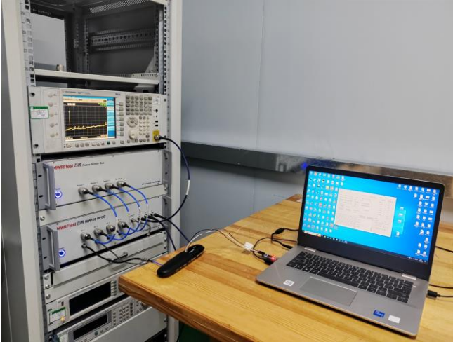
Conducted Measurement
