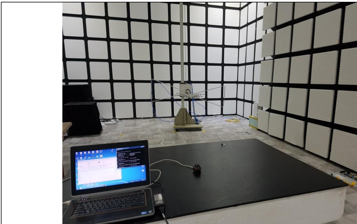
Radiated Test (Below 1G)
