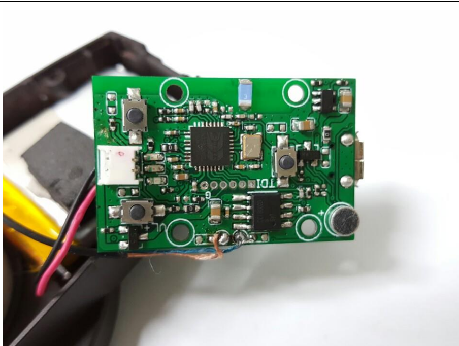
Board (Top)
