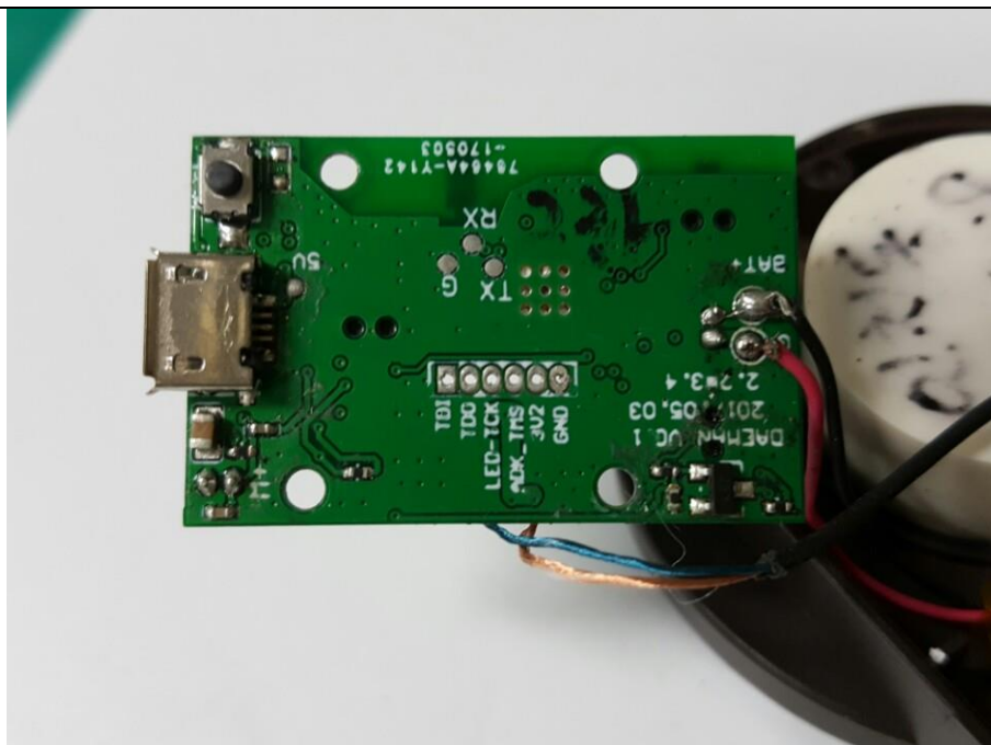
Board (Bottom)
