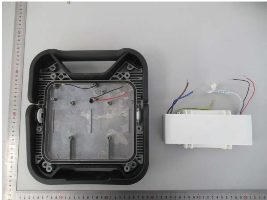
EUT – LED Driver View
