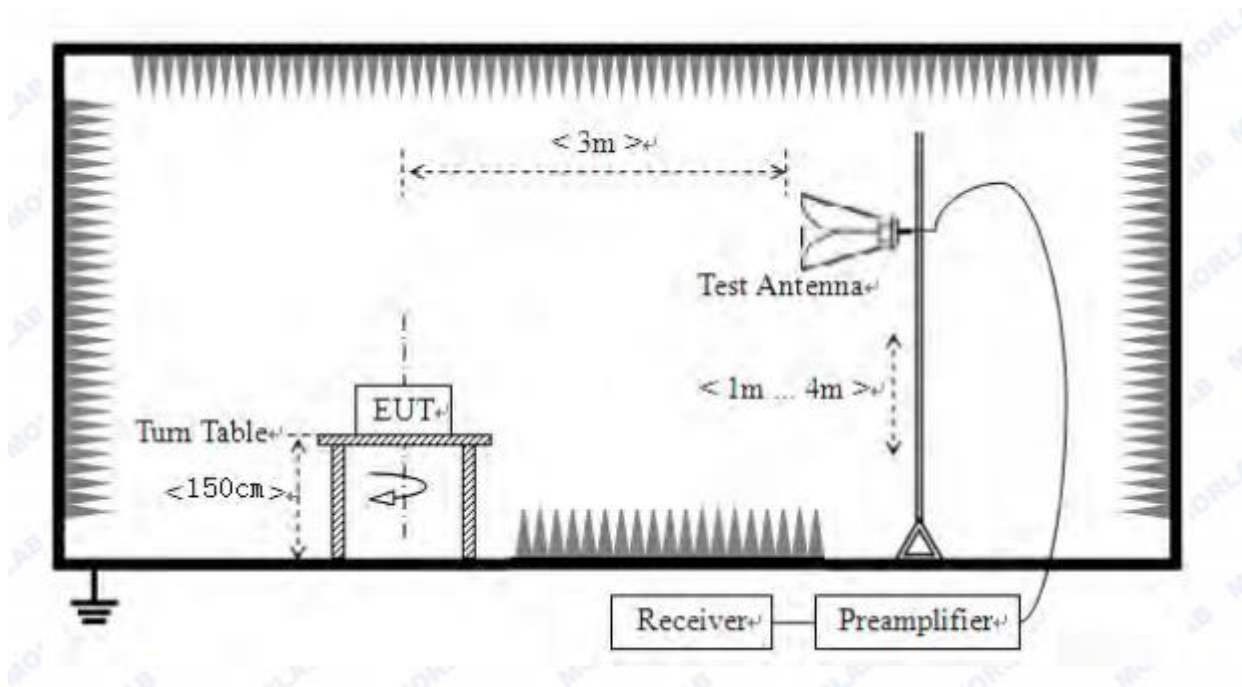
Above 1GHz Test Setup
