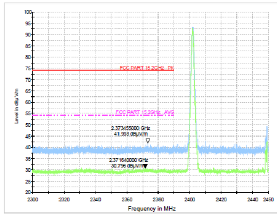
Test Mode: GFSK-Low Hopping-off
