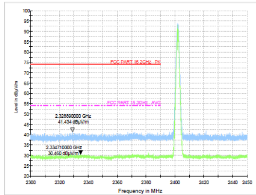
Test Mode: 8DPSK-Low Hopping-off
