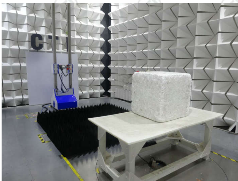
Radiated spurious emission Test Setup-1 (Above 1GHz )
