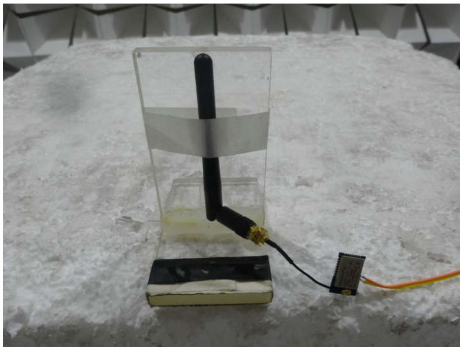
Radiated spurious emission Test Setup-2 (Above 1GHz close-up)
