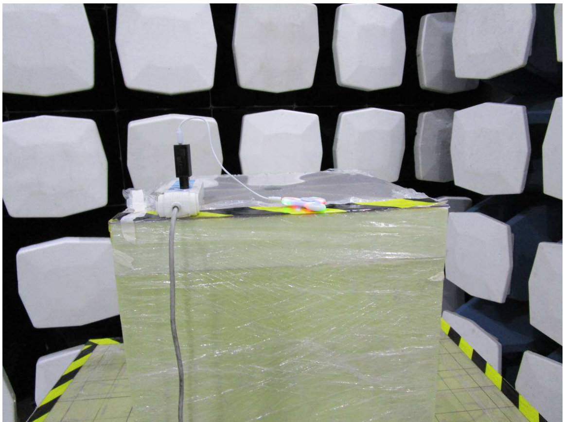
Above to 1GHz
