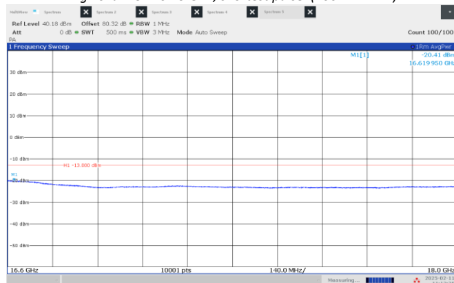
Figure 8.4-63: Emission mask, beyond \pm 250\% of BW (high frequency range), High channel: 16.45 GHz, shortest pulse. (100 MHz BW)
