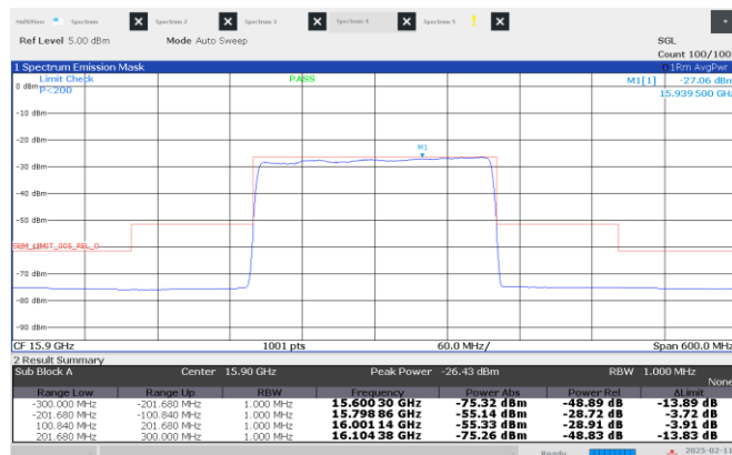
Figure 8.4-65: Emission mask, Low channel: 15.90 GHz, shortest pulse. (200 MHz BW)
