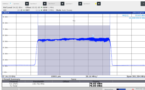
Figure 8.3-11: EIRP Power, Middle channel: 16.15 GHz, longest pulse (200 MHz BW)
