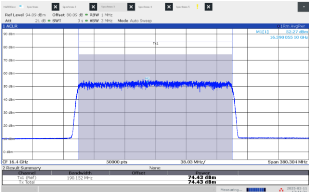
Figure 8.3-24: EIRP Power, High channel: 16.40 GHz, shortest pulse (200 MHz BW)
