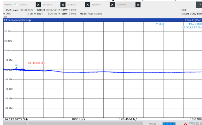
Figure 8.4-15: Emission mask, beyond \pm 250\% of BW (high frequency range), Middle channel: 16.15 GHz, longest pulse. (50 MHz BW)
