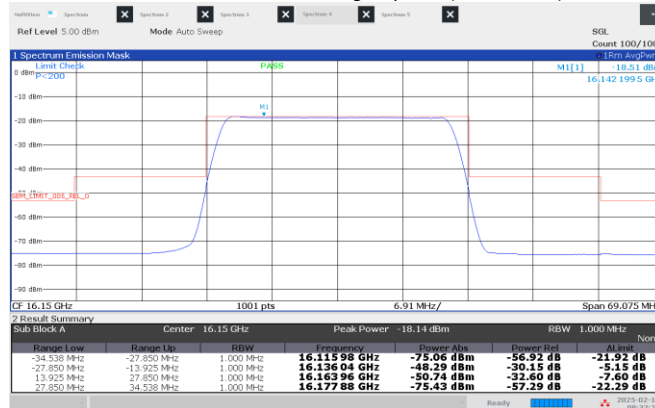
Figure 8.4-5: Emission mask, Middle channel: 16.15 GHz, longest pulse. (25 MHz BW)
