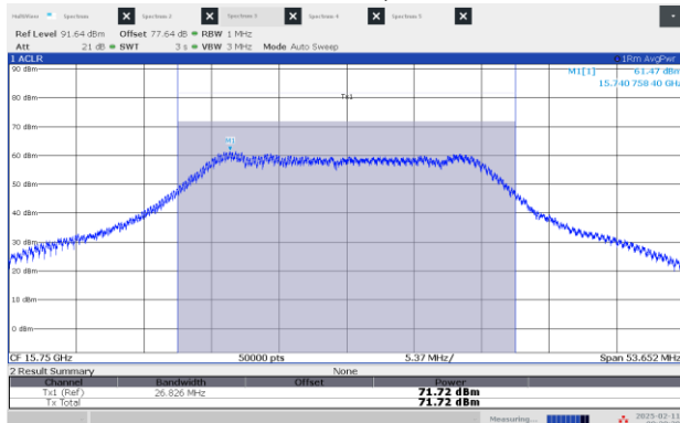
Figure 8.3-13: EIRP Power, Low channel: 15.75 GHz, shortest pulse (25 MHz BW)
