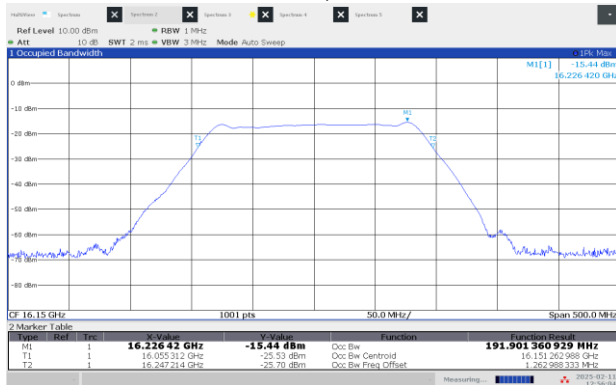
Figure 8.1-23: 99% OBW Middle channel: 16.15 GHz, shortest pulse (200 MHz BW)
