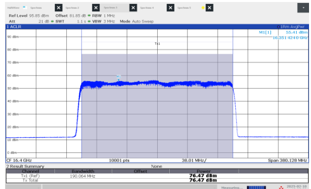
Figure 8.3-12: EIRP Power, High channel: 16.40 GHz, longest pulse (200 MHz BW)
