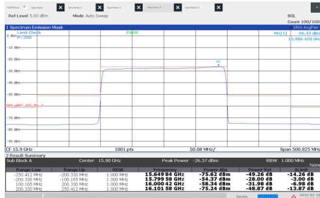
Figure 8.4-29: Emission mask, Low channel: 15.90 GHz, longest pulse. (200 MHz BW)
