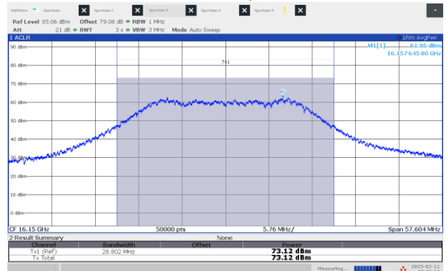
Figure 8.3-14: EIRP Power, Middle channel: 16.15 GHz, shortest pulse (25 MHz BW)
