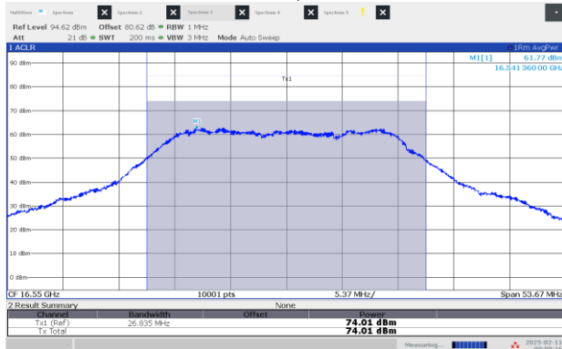
Figure 8.3-15: EIRP Power, High channel: 16.55 GHz, shortest pulse (25 MHz BW)
