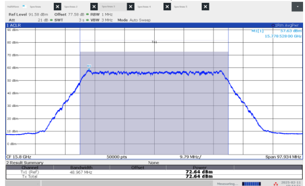
Figure 8.3-16: EIRP Power, Low channel: 15.80 GHz, shortest pulse (50 MHz BW)
