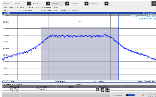
Figure 8.3-11: EIRP Power, High channel: 15.65 GHz, shortest pulse (25 MHz BW)
