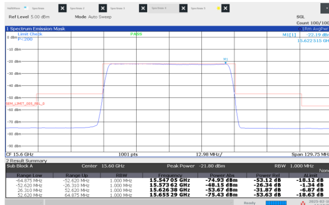
Figure 8.4-17: Emission mask, High channel: 15.60 GHz, longest pulse. (50 MHz BW)
