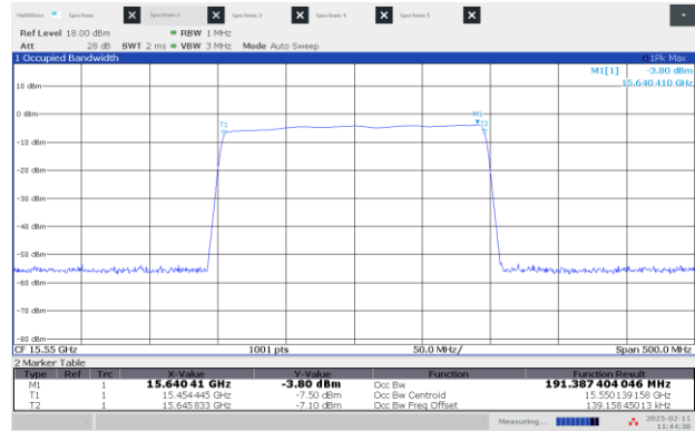
Figure 8.1-16: 99% OBW Middle channel: 15.55 GHz, shortest pulse (200 MHz BW)
