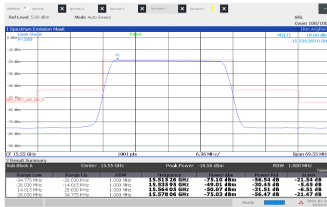
Figure 8.4-5: Emission mask, Middle channel: 15.55 GHz, longest pulse. (25 MHz BW)
