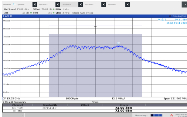
Figure 8.3-13: EIRP Power, Middle channel: 15.55 GHz, shortest pulse (50 MHz BW)
