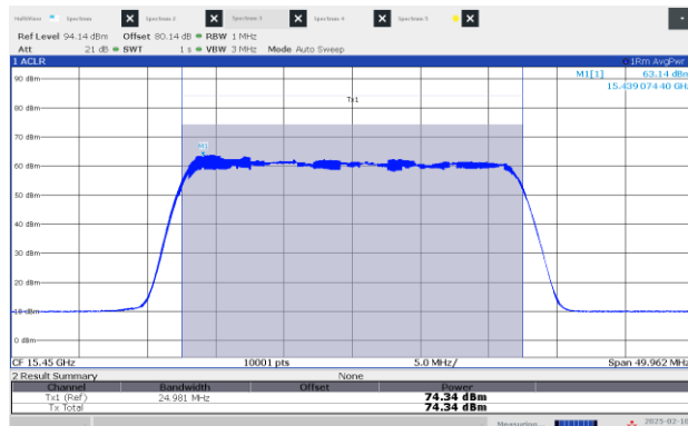
Figure 8.3-1: EIRP Power, Low channel: 15.45 GHz, longest pulse (25 MHz BW)
