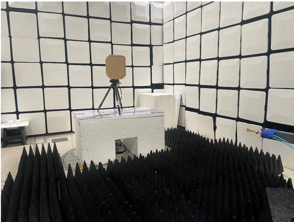
Figure 16 - Radiated emissions above 1 GHz (75 – 100 GHz), front view.
