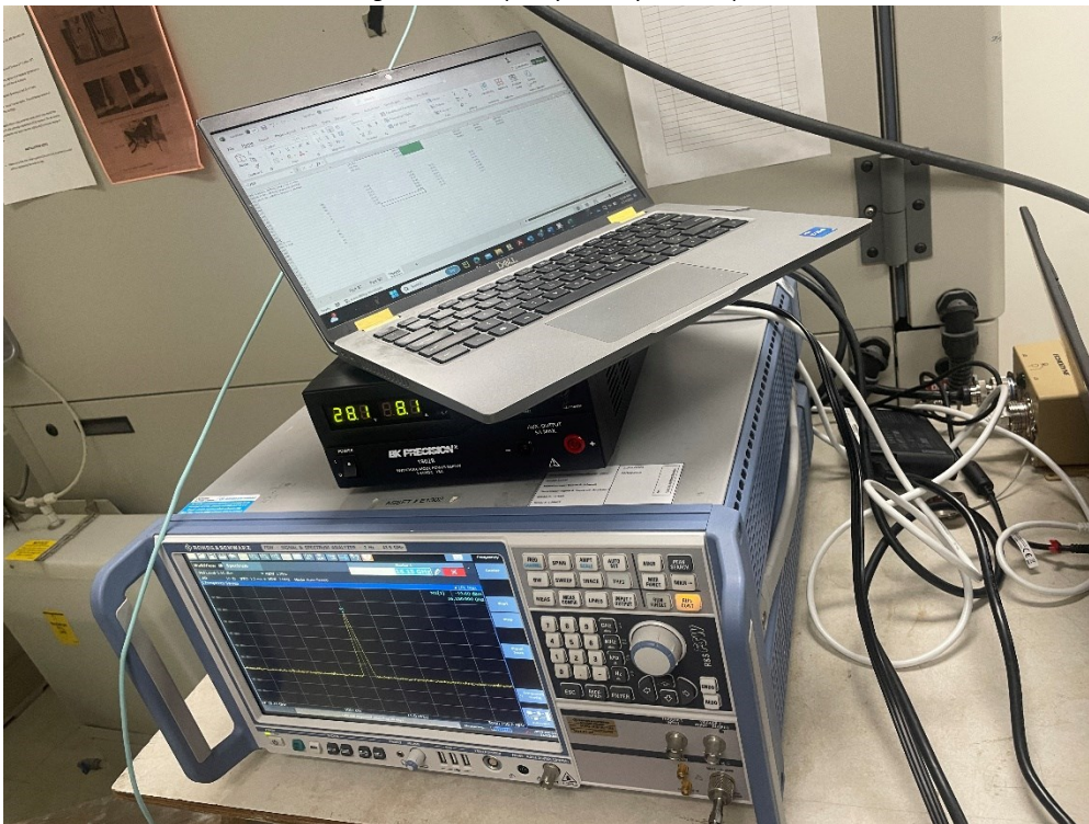
Figure 19 – Frequency stability test setup
