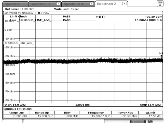
Figure 8.4-70: Emission mask, beyond \pm 250\% of BW (low frequency range), High channel: 16.40 GHz, shortest pulse. (200 MHz BW)
