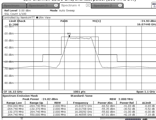
Figure 8.4-68: Emission mask, Middle channel: 16.15 GHz, shortest pulse. (200 MHz BW)
