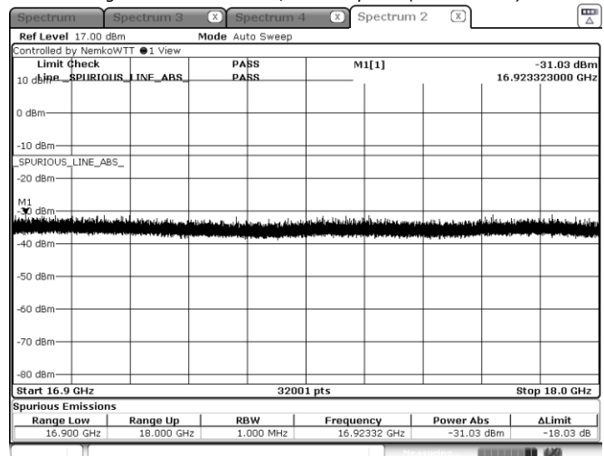
Figure 8.4-72: Emission mask, beyond \pm 250\% of BW (high frequency range), High channel: 16.40 GHz, shortest pulse. (200 MHz BW)
