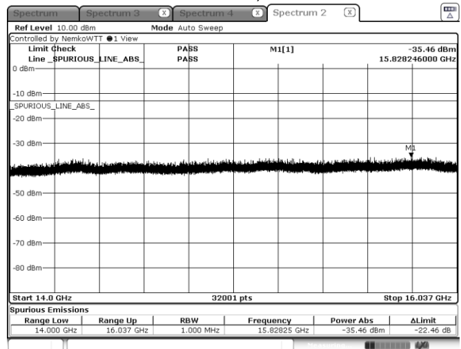
Figure 8.4-40: Emission mask, beyond \pm 250\% of BW (low frequency range), Middle channel: 16.15 GHz, shortest pulse. (25 MHz BW)
