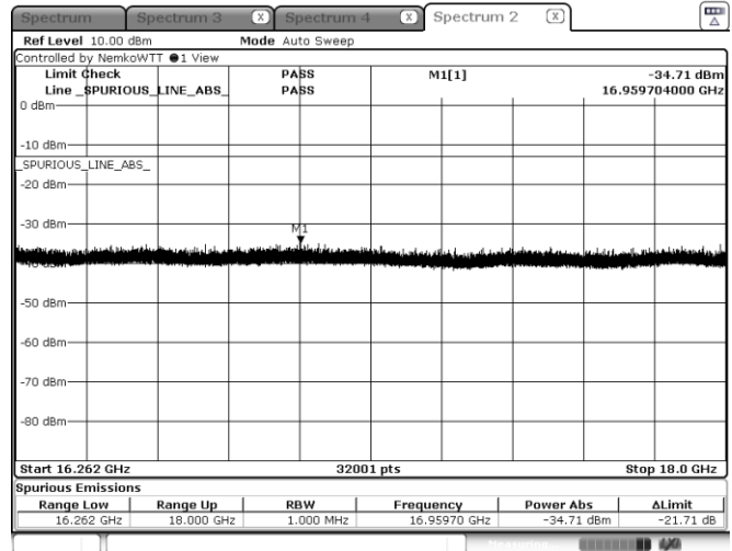
Figure 8.4-42: Emission mask, beyond \pm 250\% of BW (high frequency range), Middle channel: 16.15 GHz, shortest pulse. (25 MHz BW)
