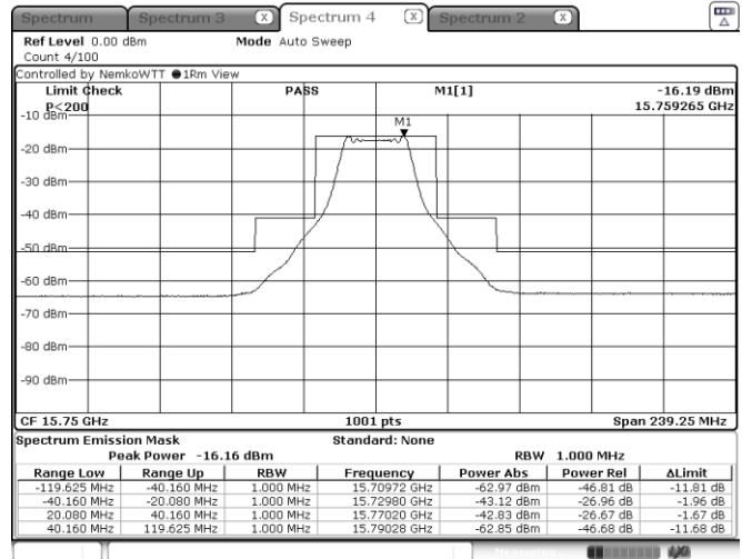
Figure 8.4-38: Emission mask, Low channel: 15.75 GHz, shortest pulse. (25 MHz BW)
