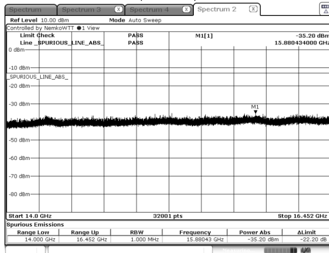
Figure 8.4-43: Emission mask, beyond \pm 250\% of BW (low frequency range), High channel: 16.55 GHz, shortest pulse. (25 MHz BW)
