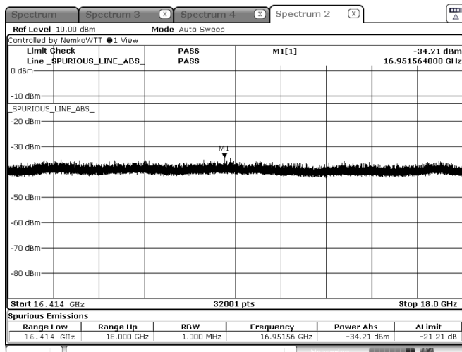
Figure 8.4-66: Emission mask, beyond \pm 250\% of BW (high frequency range), Low channel: 15.90 GHz, shortest pulse. (200 MHz BW)
