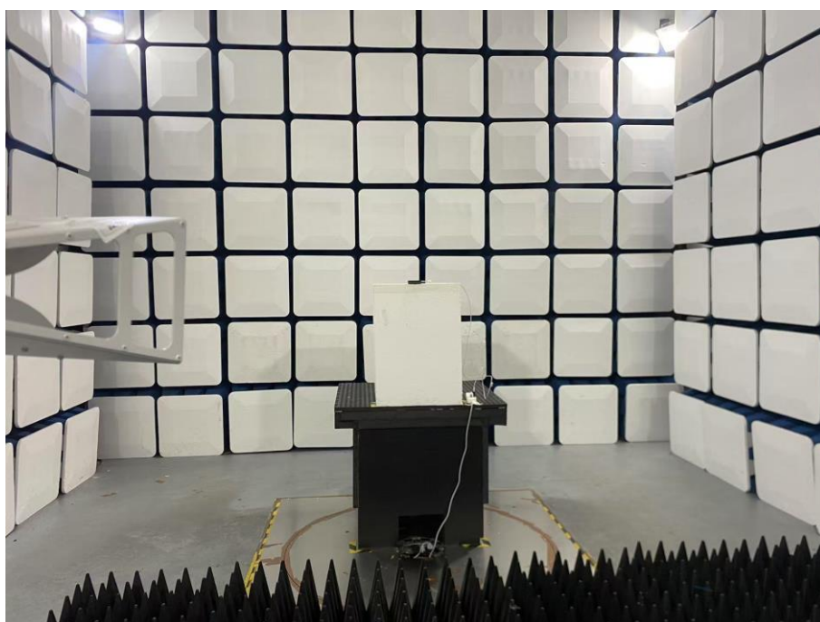
Above 1GHz-WIFI
