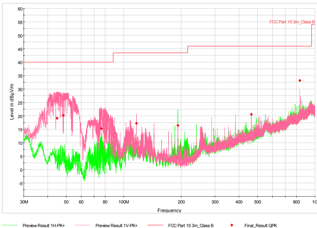
Figure 7-32: Radiated Emissions - 30 MHz to 1 GHz (§ 15.205, 15.209) – Configuration 5
