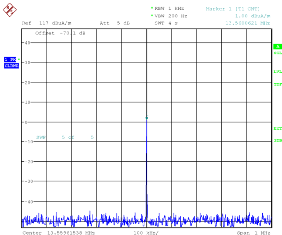
Figure 7-39: Frequency stability – 20 °C / 5 V at startup – Configuration 2
