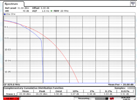
LTE Band 5 10MHz (Low Channel)-16QAM
