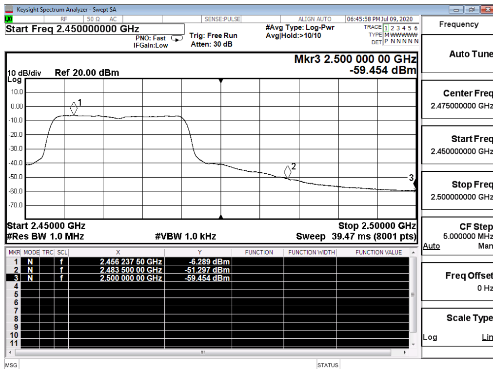
Restrict-band band-edge measurements_11G_2462_Ant1_AV
