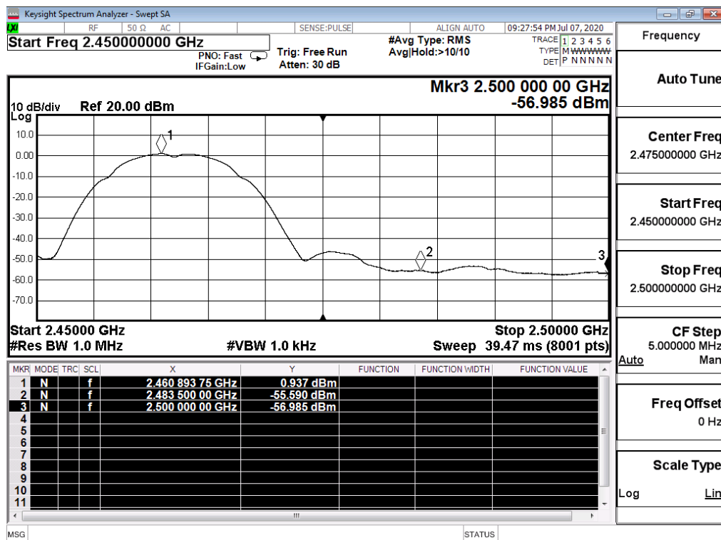
Restrict-band band-edge measurements_11B_2462_Ant1_AV
