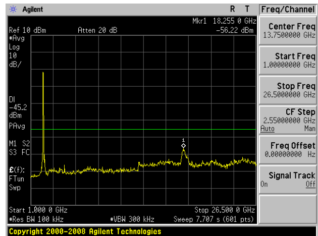
802.11n40 on channel 03
