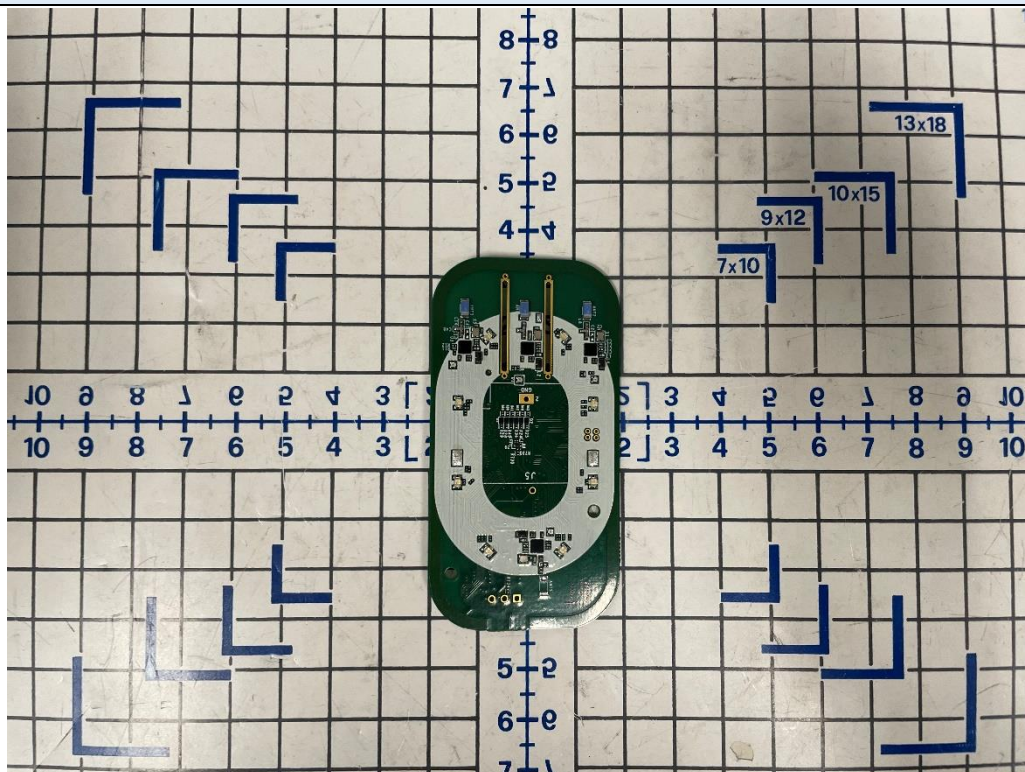
Antenna Board Front View
