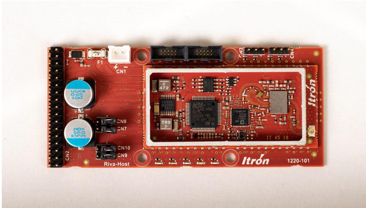
Modular-LE Front without shields
