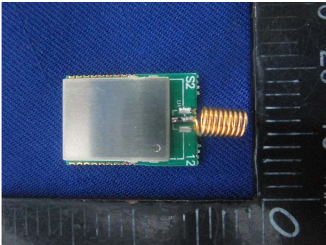
Model: RC-S2LP-915-HA
