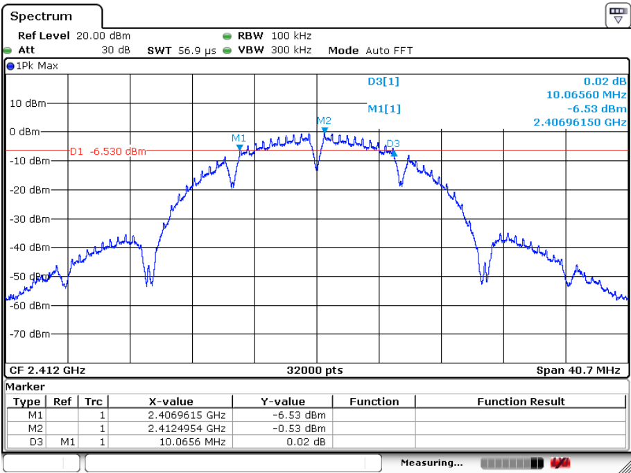
802.11b-Low Channel
