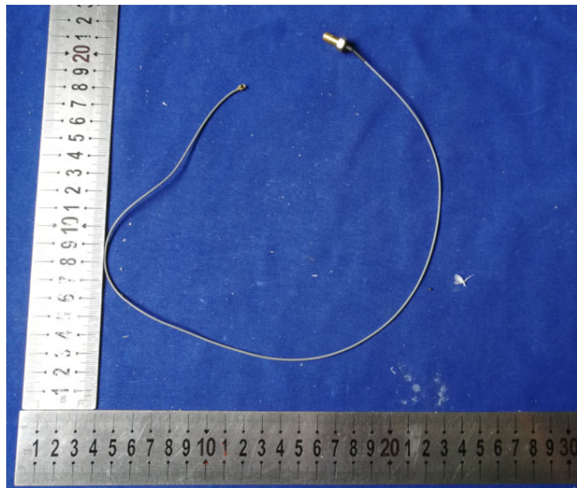
EUT – Antenna View
