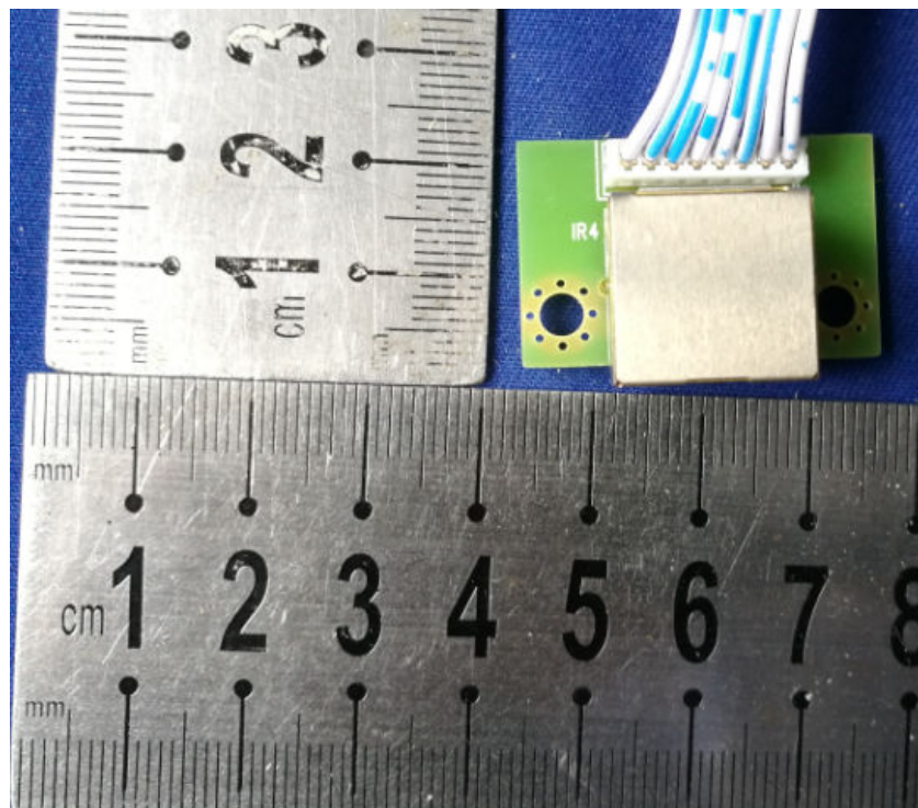
EUT – PCB View
