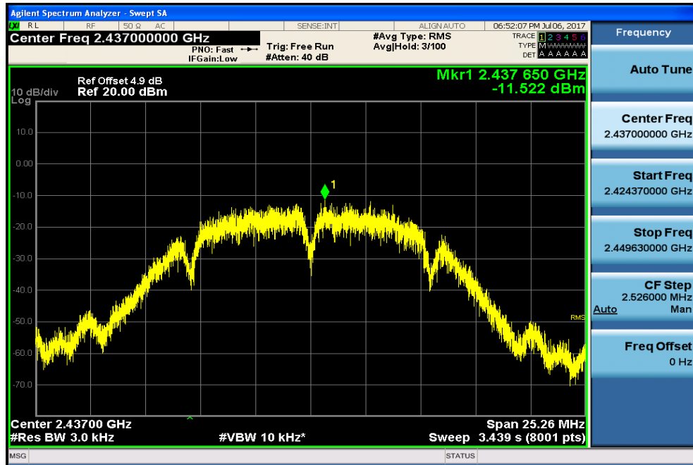
802.11b-Middle Channel
