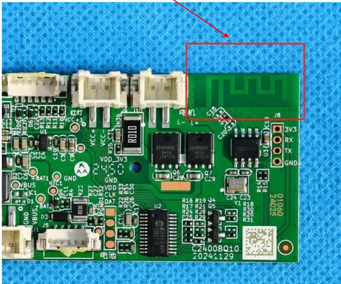
View of wireless antenna
