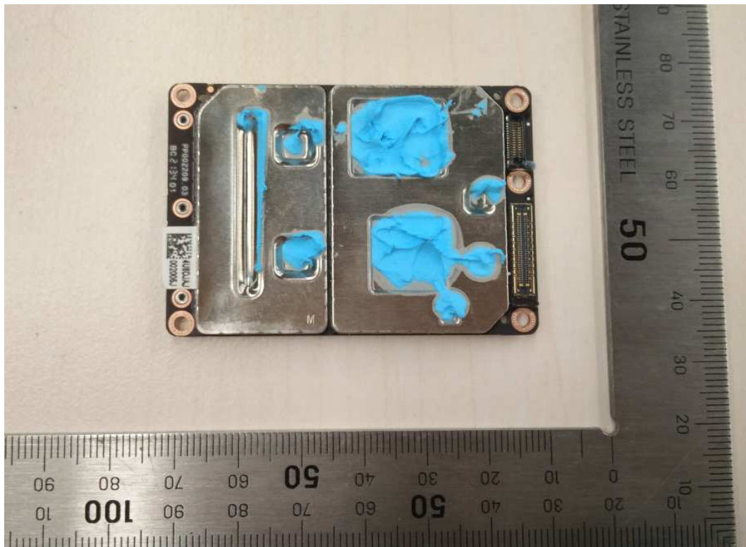
Figure 9: ANT board view -1
