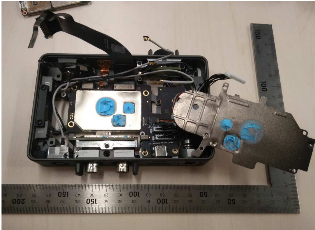
Figure 3: Internal view -3
