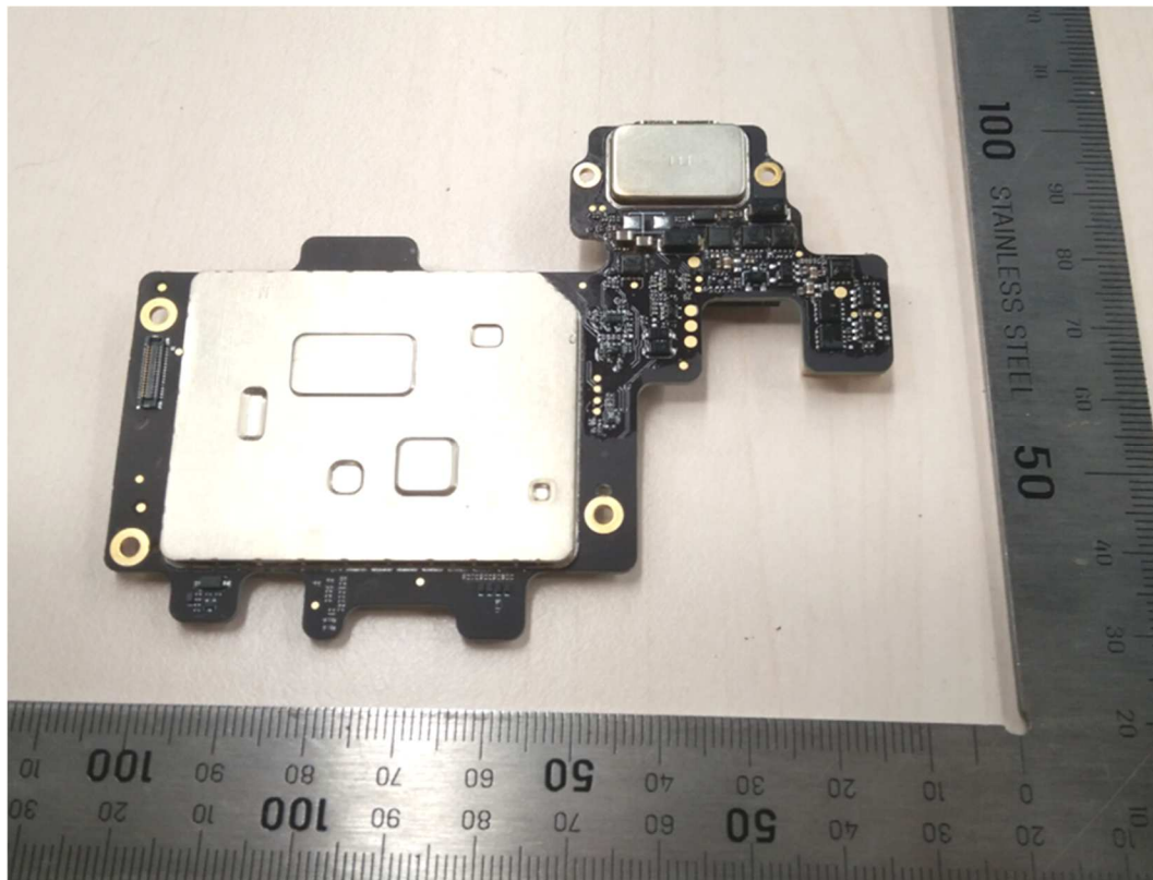
Figure 7: Mainboard view -3
