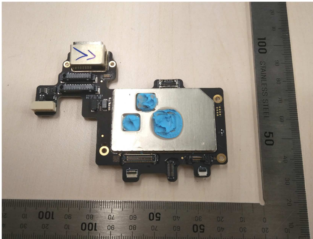
Figure 5: Mainboard view -1
