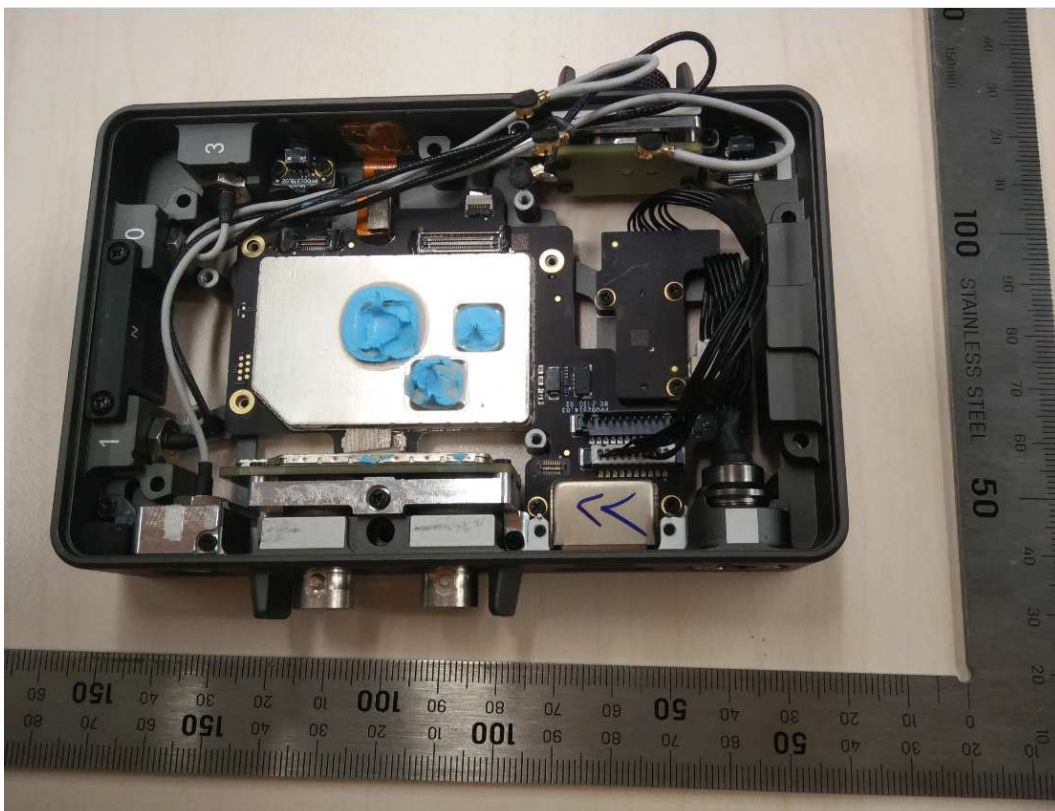
Figure 4: Internal view -4
