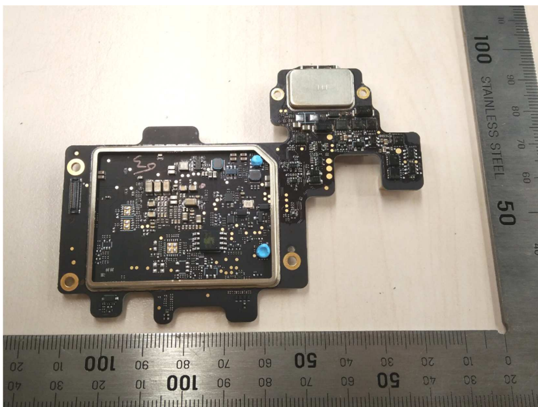
Figure 8: Mainboard view -4
