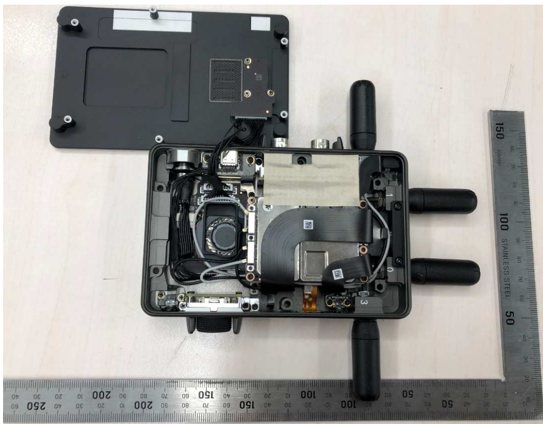
Figure 2: Internal view -2
